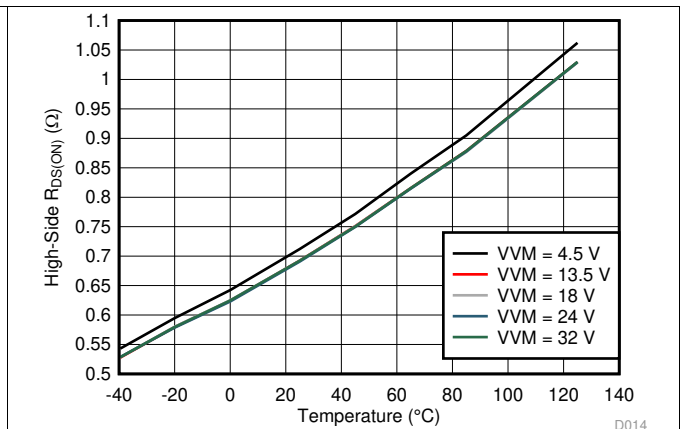
Figure 15. High Side On-State Resistance ( R_{DS(ON)} ) vs Ambient Temperature ( T_A )
