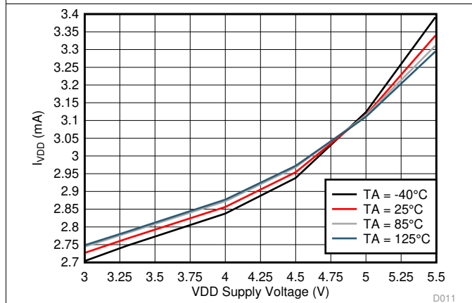
Figure 12. VDD Operating Mode Current ( I_{VDD} ) vs Supply Voltage ( V_{VDD} )
