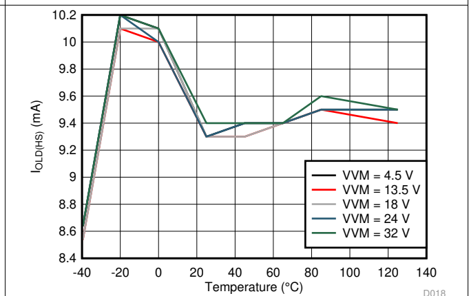
Figure 19. High-Side Open-load Detection Current ( I_{OL(D)} ) vs Ambient Temperature ( T_A )
