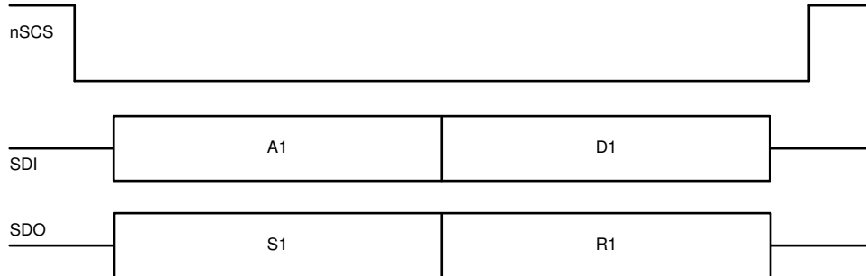
Figure 69. SPI Data Frame
