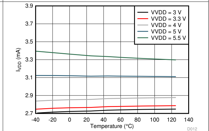
Figure 13. VDD Operating Mode Current ( I_{VDD} ) vs Ambient Temperature ( T_A )
