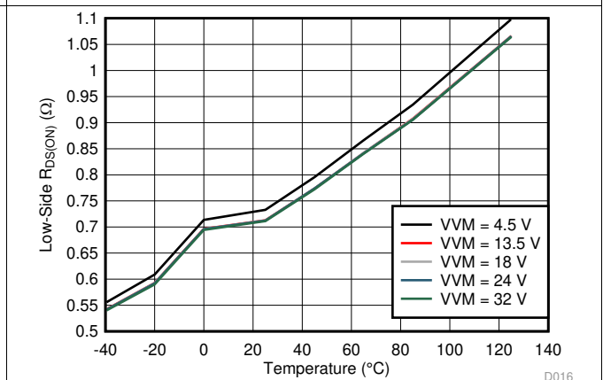
Figure 17. Low-Side On-State Resistance ( R_{DS(ON)} ) vs Ambient Temperature ( T_A )
