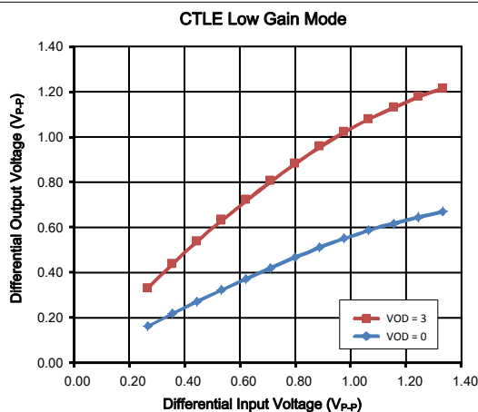
Figure 7-1. Typical Vin/Vout Linearity (straight-thru mode)
