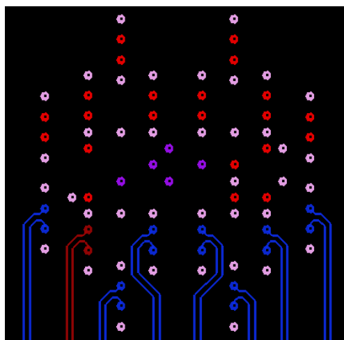
Figure 11-2. Stripline example, Internal Signal Layer 1
