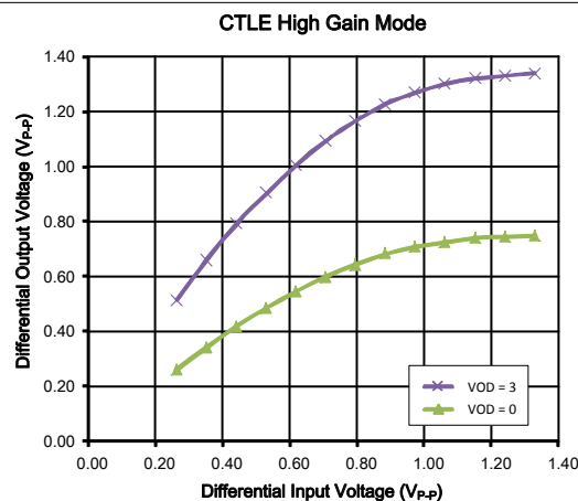
Figure 7-2. Typical Vin/Vout Linearity (straight-thru mode)
