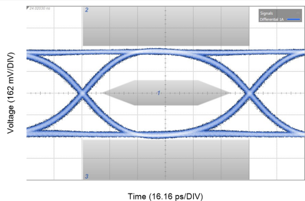
Figure 9-15. 10.3125 Gbps nPPI Eye Mask with 5 in input channel and minimal output channel
