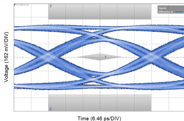
Figure 9-14. 25.78125 Gbps CAUI-4 Eye Mask with 5 in input channel and minimal output channel
