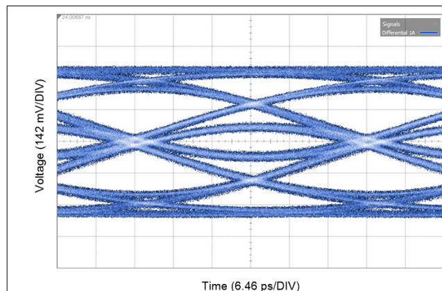
Figure 9-20. 25.78125 Gbps Eye Diagram with 10 in input channel and 5 in output channel, Linear mode
