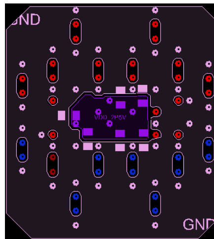
Figure 11-4. Stripline example, Bottom Layer
