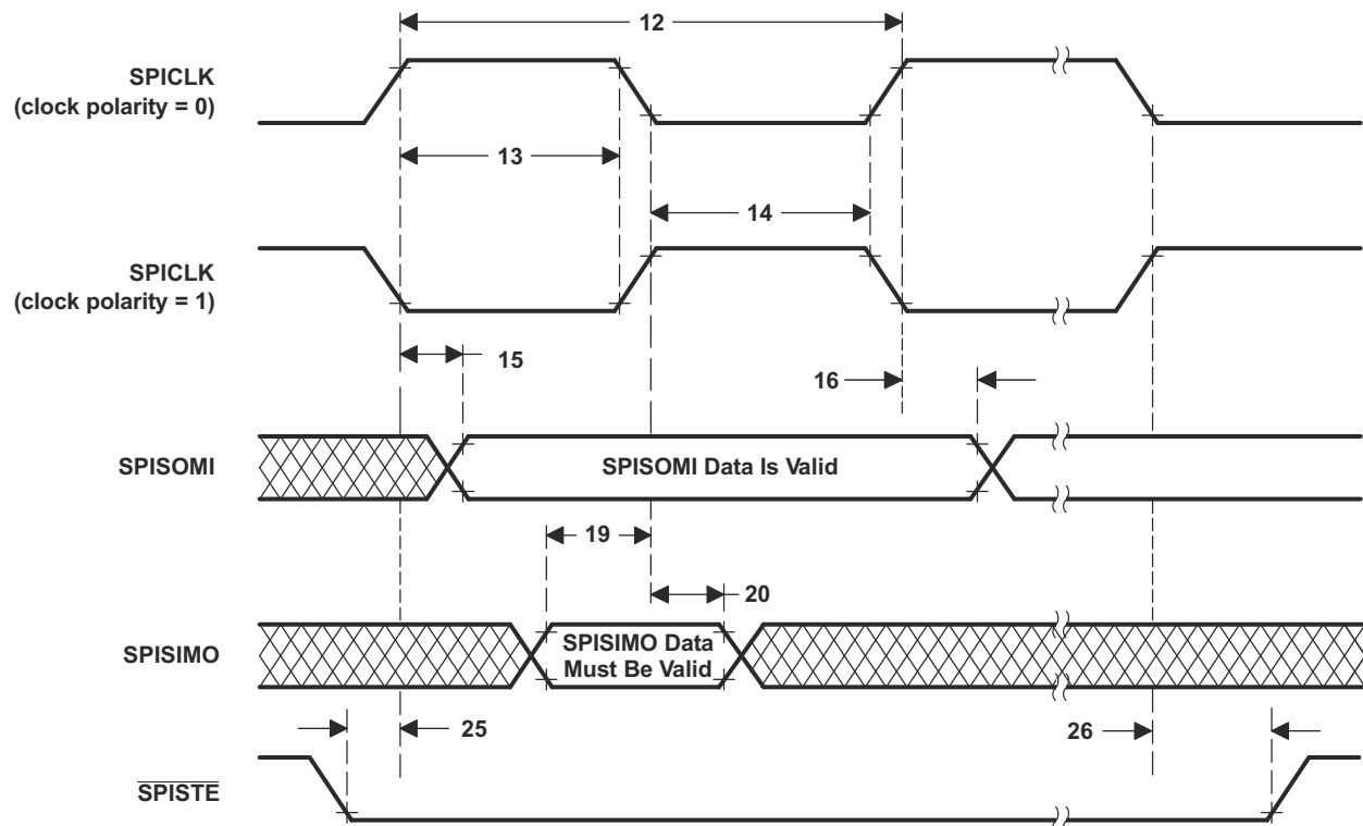
Figure 7-86. SPI Slave Mode External Timing (Clock Phase = 0)
