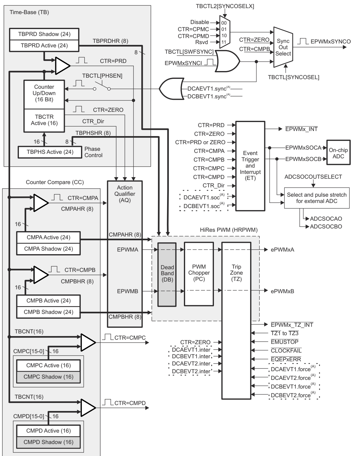
Figure 7-67. ePWM Submodules and Critical Internal Signal Interconnects
