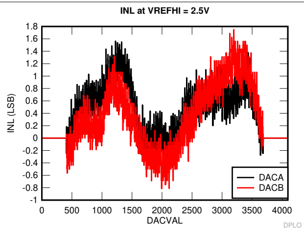
Figure 7-52. INL
