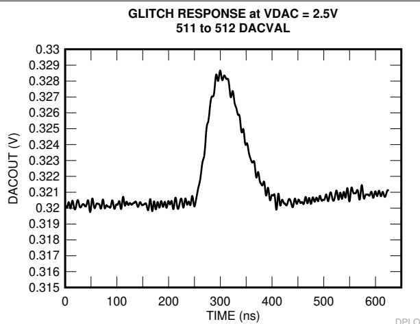
Figure 7-53. Glitch Response – 511 to 512 DACVAL
