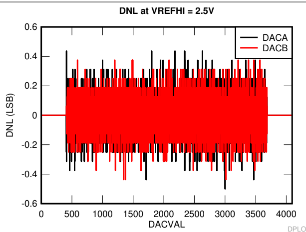
Figure 7-51. DNL
