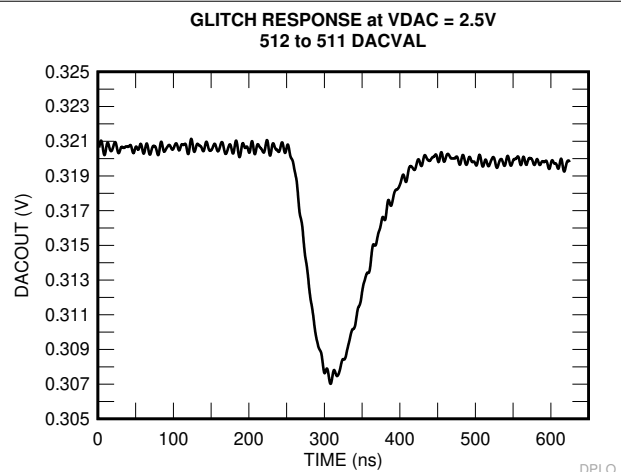
Figure 7-54. Glitch Response – 512 to 511 DACVAL
