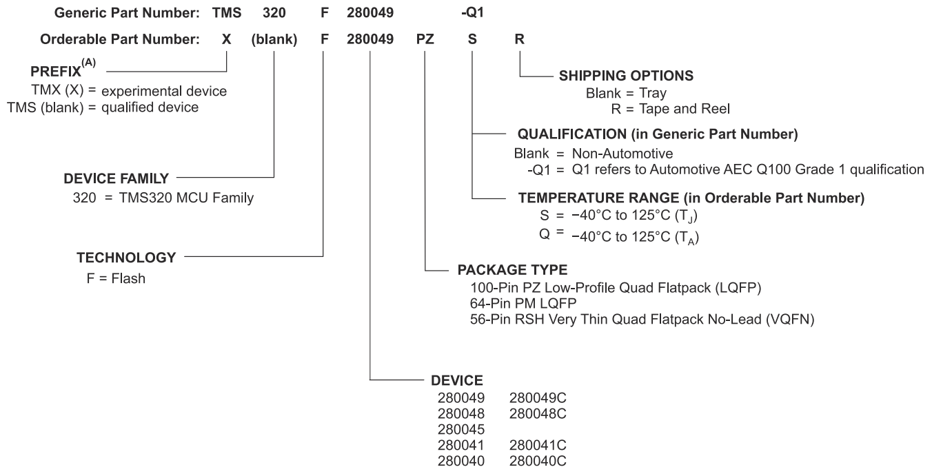
Figure 10-1. Device Nomenclature
