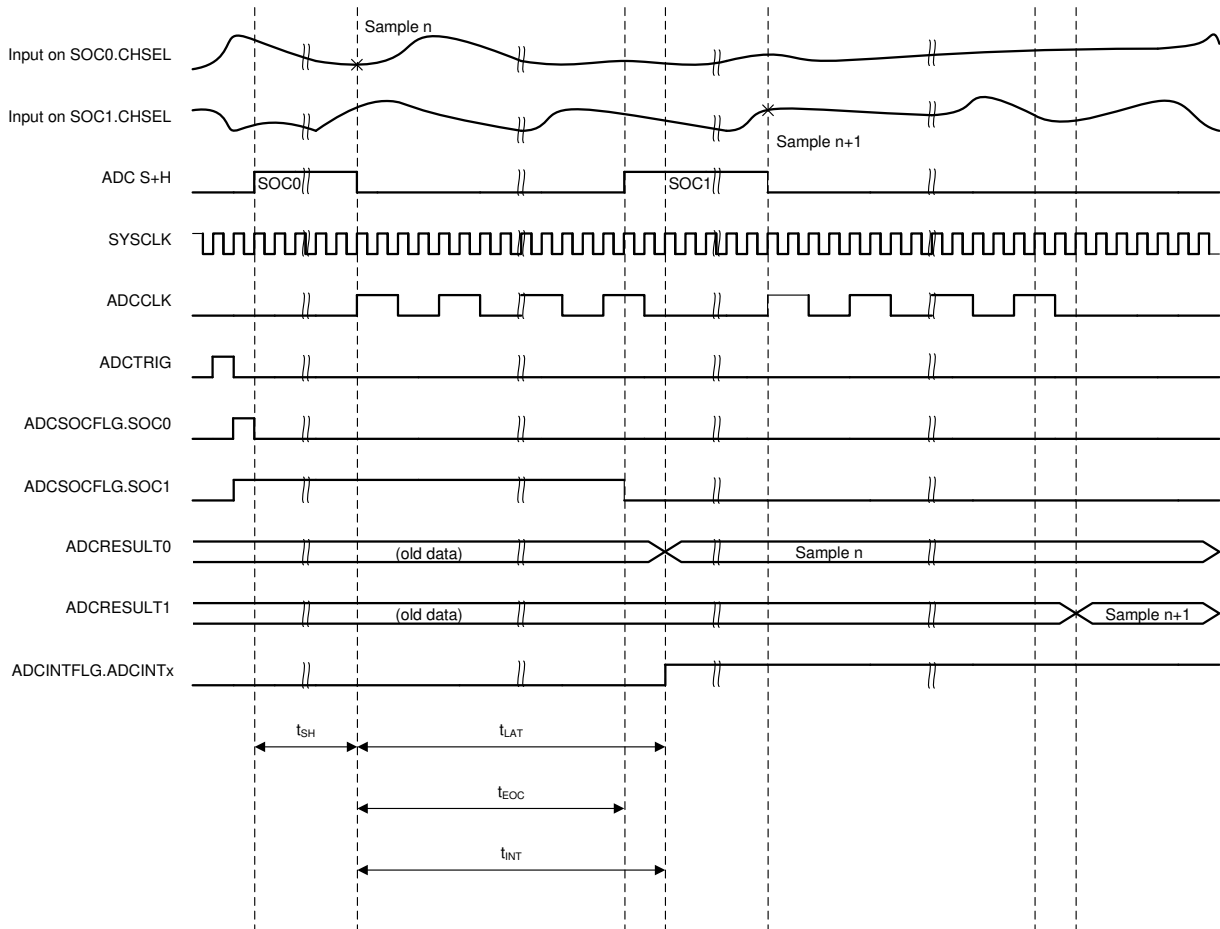
Figure 7-44. ADC Timings
