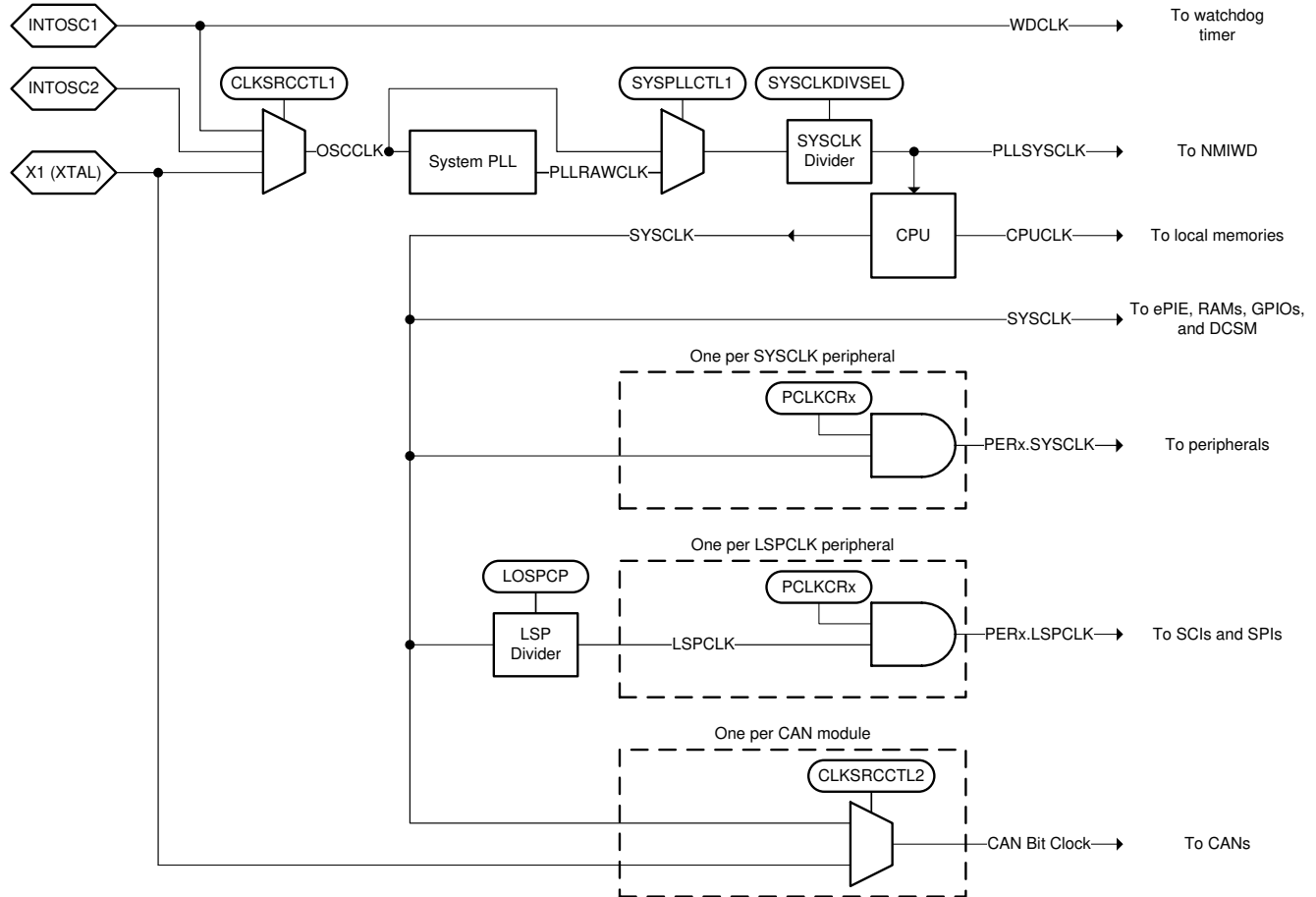
Figure 7-15. Clocking System
