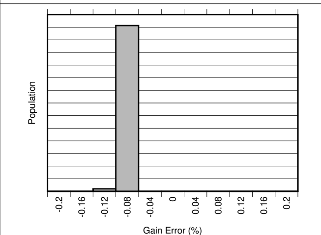
Figure 6-12. Gain Error Distribution (INA301A3-Q1)
