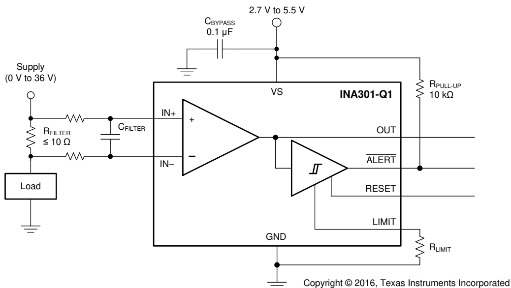
Figure 8-1. Input Filter
