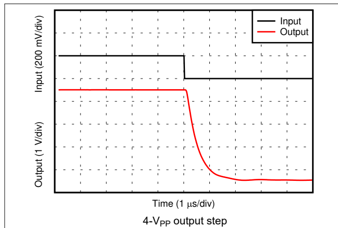
Figure 6-25. Voltage Output Falling Step Response
