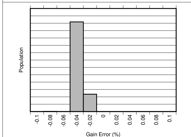
Figure 6-11. Gain Error Distribution (INA301A2-Q1)
