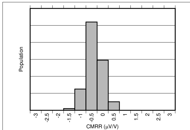
Figure 6-7. Common-Mode Rejection Ratio Distribution (INA301A3-Q1)
