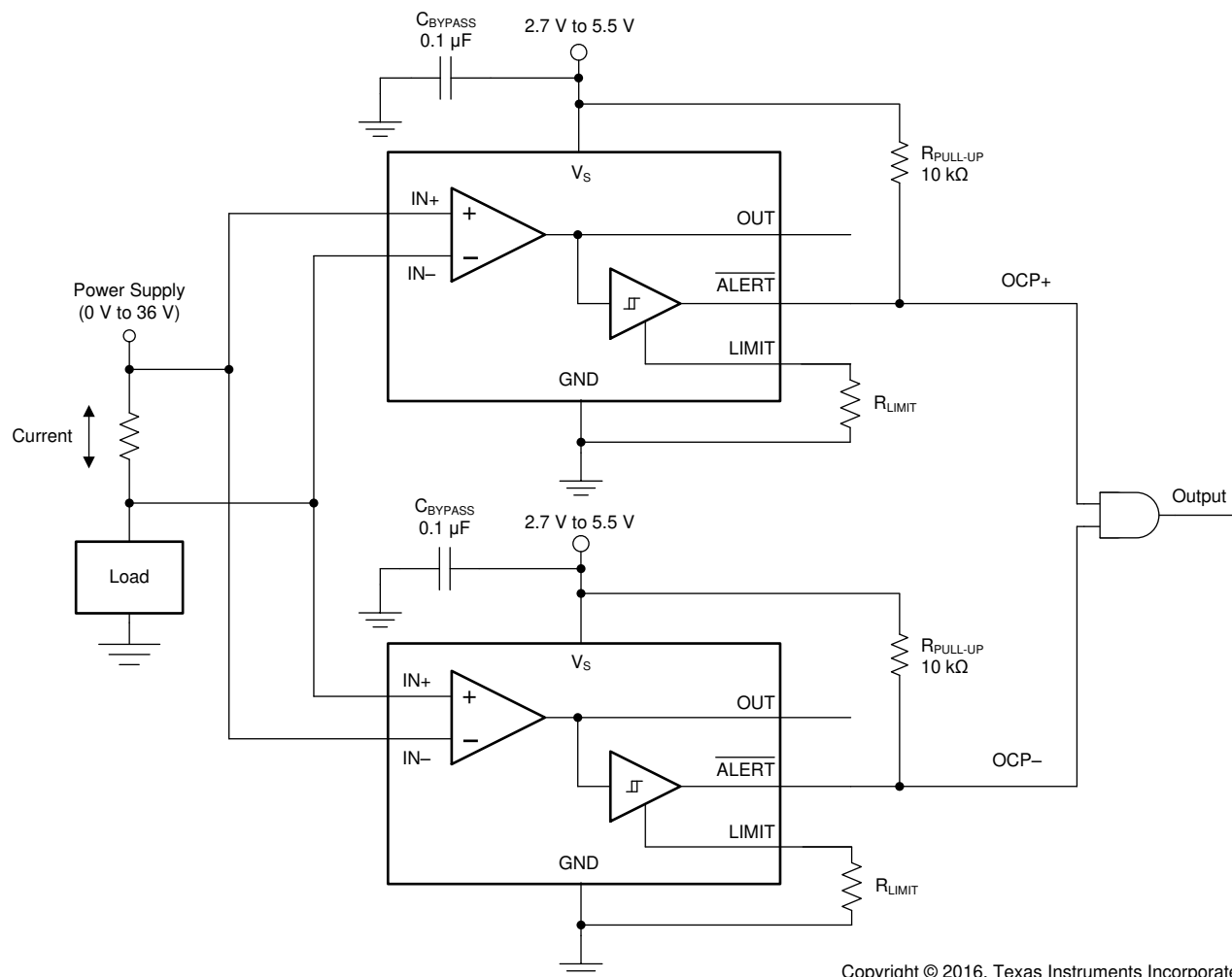
Figure 8-4. Bidirectional Application
