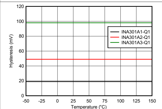
Figure 6-34. Hysteresis vs. Temperature
