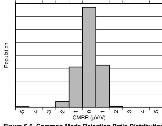
Figure 6-6. Common-Mode Rejection Ratio Distribution (INA301A2-Q1)
