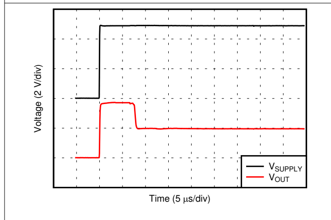
Figure 6-27. Start-Up Response
