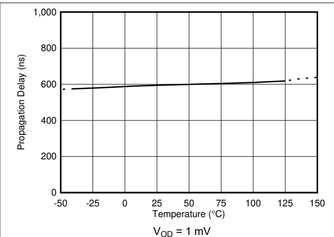
Figure 6-32. Comparator Propagation Delay vs. Temperature
