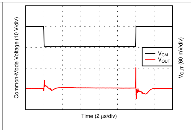
Figure 6-26. Common-Mode Voltage Transient Response
