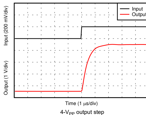
Figure 6-24. Voltage Output Rising Step Response
