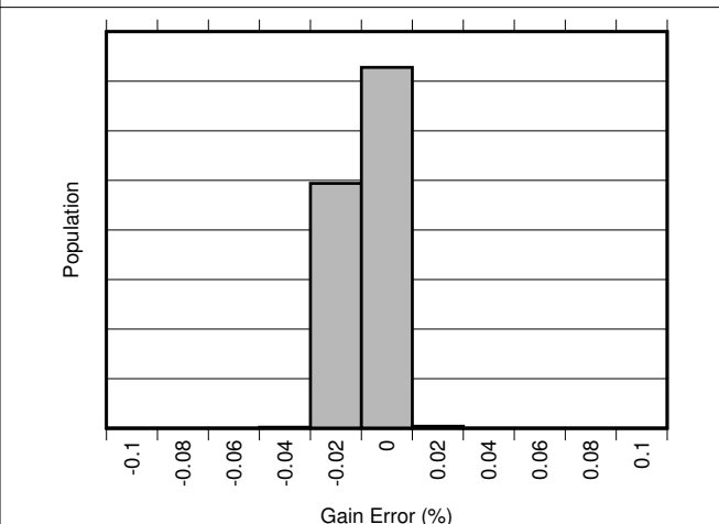
Figure 6-10. Gain Error Distribution (INA301A1-Q1)
