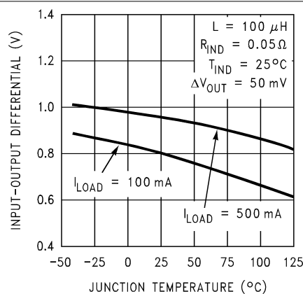
Figure 7-6. Dropout Voltage
