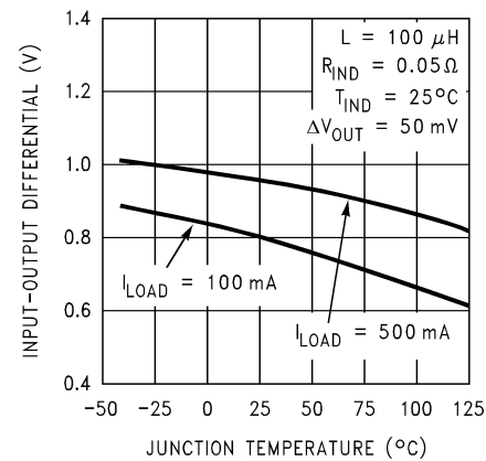
Figure 7-6. Dropout Voltage
