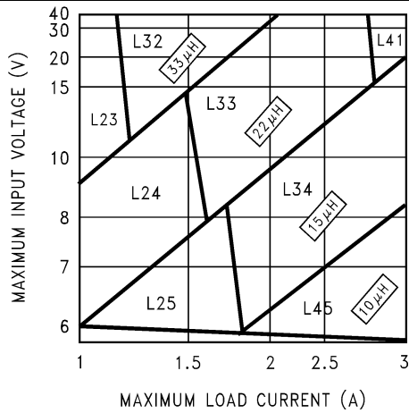
Figure 17. LM2670 – 3.3 V
