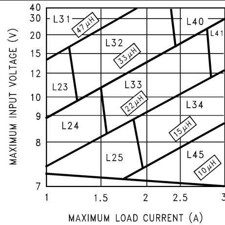
Figure 18. LM2670 – 5 V
