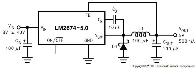
Figure 7-9. Typical Application
