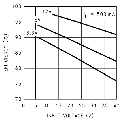
Figure 5-3. Efficiency
