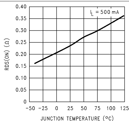
Figure 5-4. Drain-to-Source Resistance
