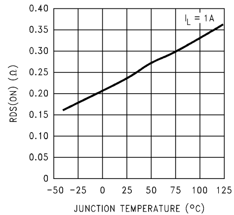
Figure 5-4. Drain-to-Source Resistance
