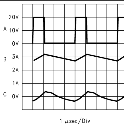
Figure 5-10. Switching Frequency
