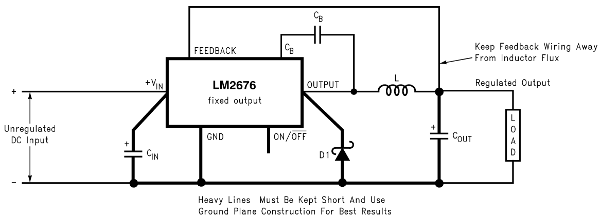
Figure 7-6. Basic Circuit for Fixed Output Voltage Applications.
