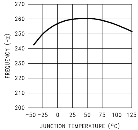
Figure 5-10. Switching Frequency
