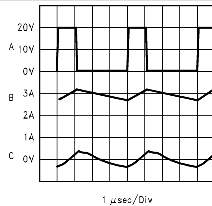
Figure 5-10. Switching Frequency
