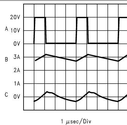
Figure 5-10. Switching Frequency
