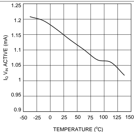
Figure 2. I_{q, V_{IN} \text{ (Active)}} vs Temperature - Y Option
