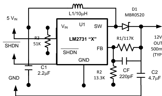
Figure 24. Application Schematic
