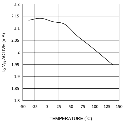
Figure 1. I_{q, V_{IN} \text{ (Active)}} vs Temperature - X Option
