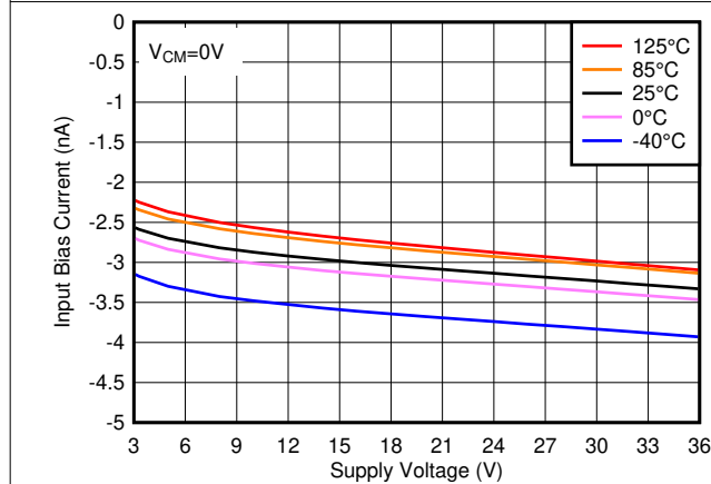
Figure 5-15. Input Bias Current vs. Supply Voltage
