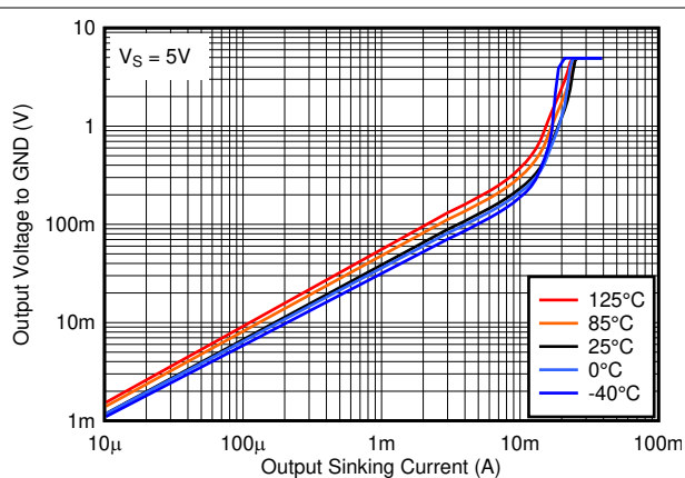
Figure 2-20. Output Low Voltage vs. Output Sinking Current at 5V
