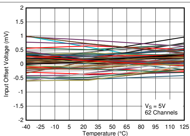
Figure 2-8. Input Offset Voltage vs. Temperature at 5V
