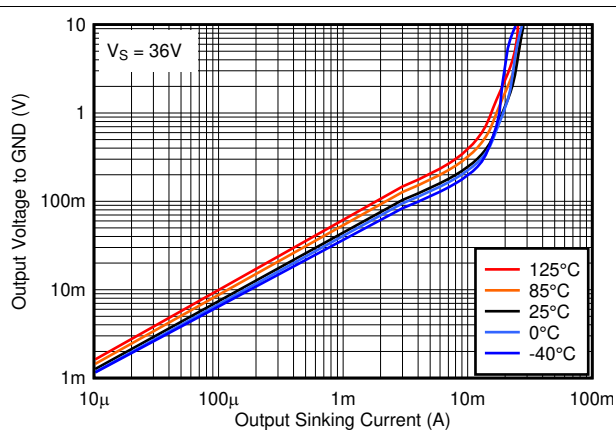
Figure 2-22. Output Low Voltage vs. Output Sinking Current at 36V
