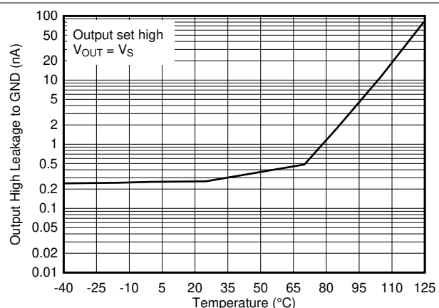
Figure 2-24. Output High Leakage Current vs. Temperature at 36V
