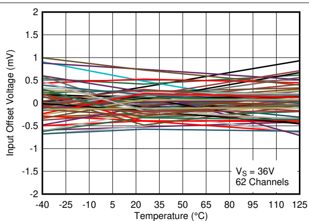
Figure 2-10. Input Offset Voltage vs. Temperature at 36V
