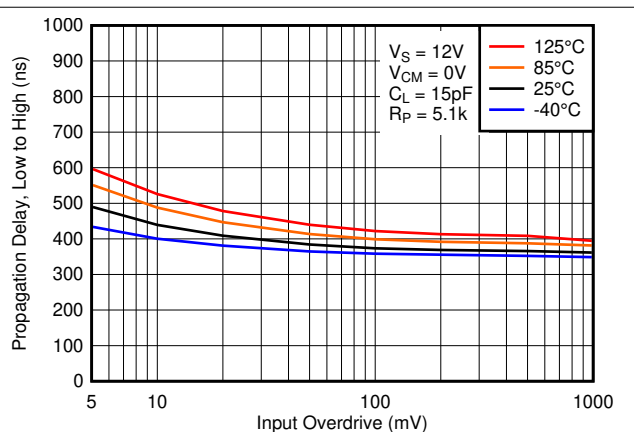
Figure 2-28. Low to High Propagation Delay vs. Input Overdrive Voltage, 12V
