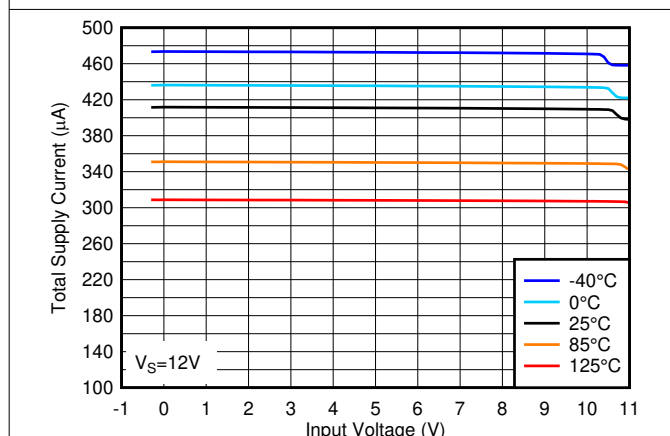
Figure 2-5. Total Supply Current vs. Input Voltage at 12V
