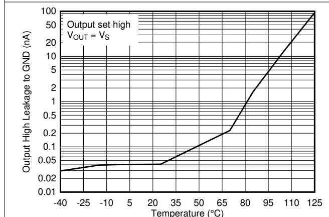
Figure 2-23. Output High Leakage Current vs. Temperature at 5V
