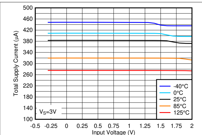
Figure 2-2. Total Supply Current vs. Input Voltage at 3V
