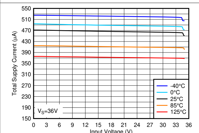
Figure 2-6. Total Supply Current vs. Input Voltage at 36V
