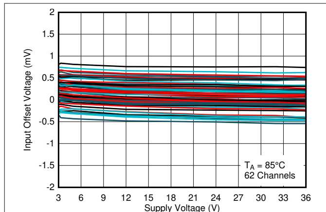
Figure 2-13. Input Offset Voltage vs. Supply Voltage at 85°C
