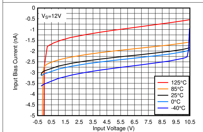
Figure 2-17. Input Bias Current vs. Input Voltage at 12V
