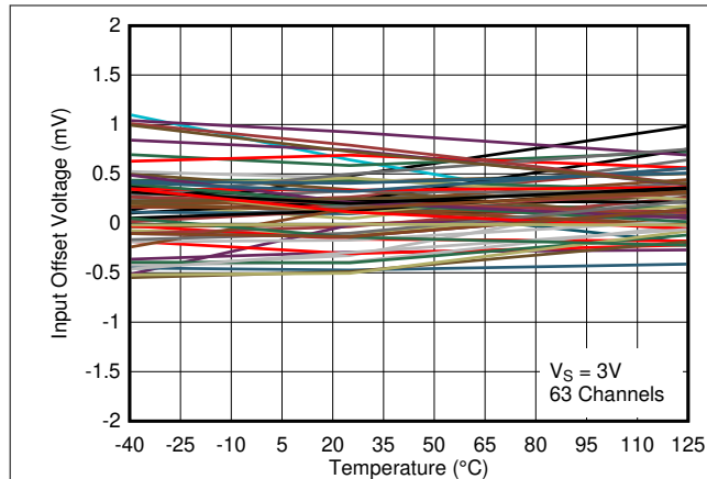
Figure 2-7. Input Offset Voltage vs. Temperature at 3V
