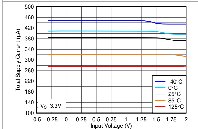
Figure 2-3. Total Supply Current vs. Input Voltage at 3.3V
