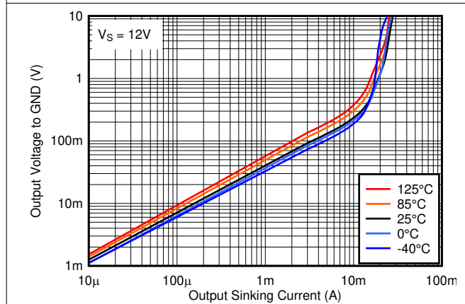
Figure 2-21. Output Low Voltage vs. Output Sinking Current at 12V
