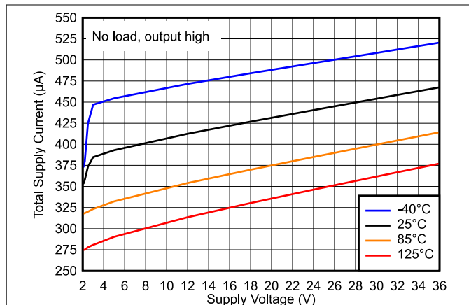
Figure 2-1. Total Supply Current vs. Supply Voltage
