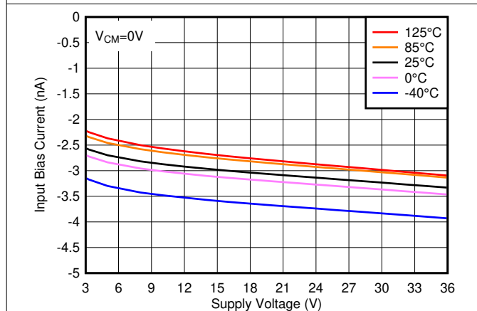
Figure 2-15. Input Bias Current vs. Supply Voltage
