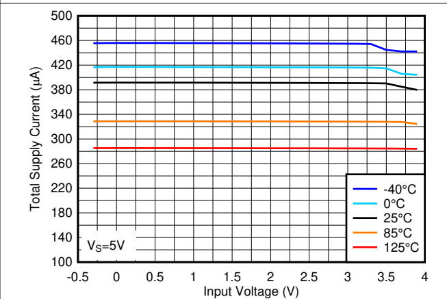
Figure 2-4. Total Supply Current vs. Input Voltage at 5V
