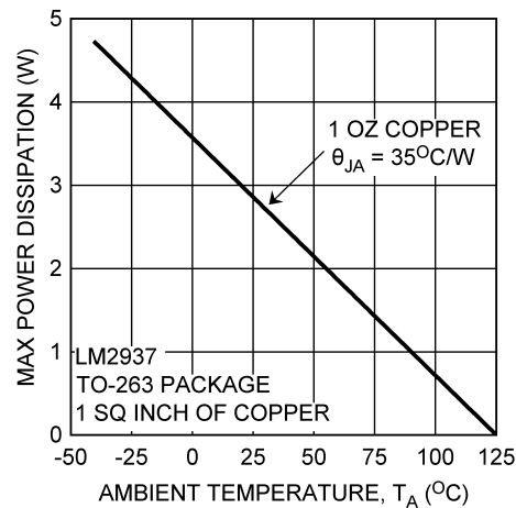
Figure 22. Maximum Power Dissipation vs. T_{AMB} for the DDPK/TO-263 Package
