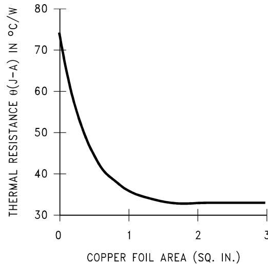
Figure 21. R_{\theta JA} vs. Copper (1 ounce) Area for the DDPK/TO-263 Package
