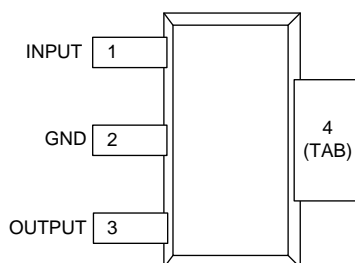
DDPAK/TO-263 Surface-Mount Package (KTT)
