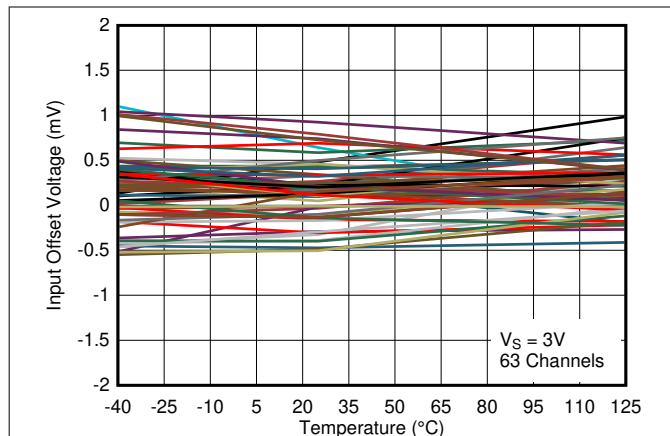
Figure 5-7. Input Offset Voltage vs. Temperature at 3V
