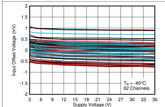
Figure 5-11. Input Offset Voltage vs. Supply Voltage at -40^\circ\text{C}
