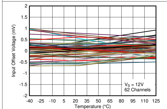
Figure 5-9. Input Offset Voltage vs. Temperature at 12V
