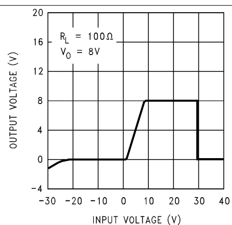
Figure 29. Output at Voltage Extremes
