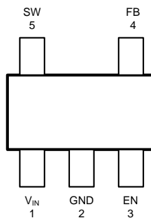
Figure 3. Top View SOT-23 Package
