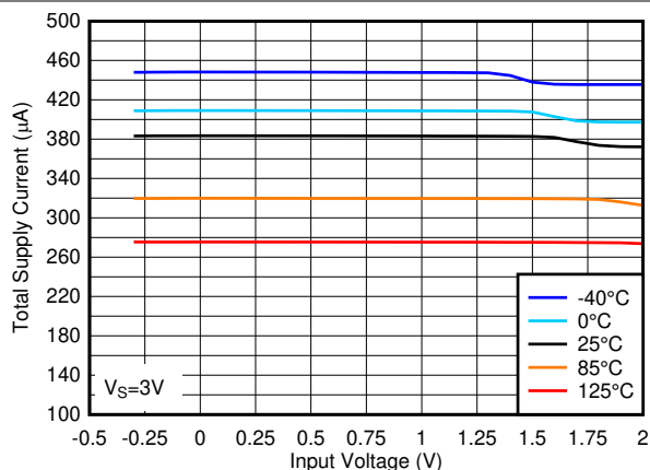
Figure 5-2. Total Supply Current vs. Input Voltage at 3V
