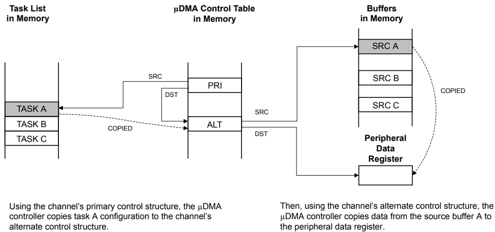
Figure 7-6. Peripheral Scatter-Gather, \mu DMA Copy Sequence
