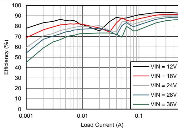
Figure 1. Efficiency
