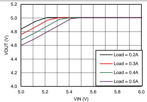
Figure 14. Dropout Curve
