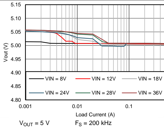
Figure 67. Output Voltage Regulation
