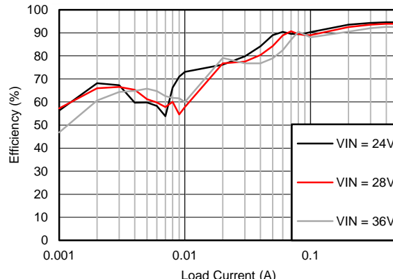
Figure 84. Efficiency
