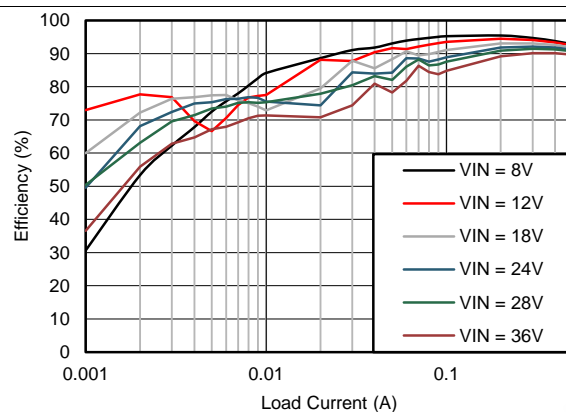
Figure 2. Efficiency
