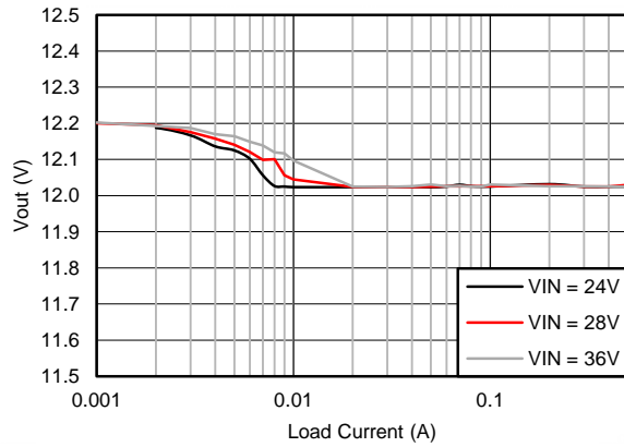
Figure 9. V_{OUT} Regulation
