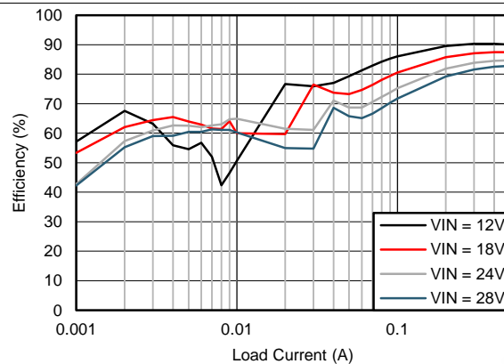
Figure 2. Efficiency
