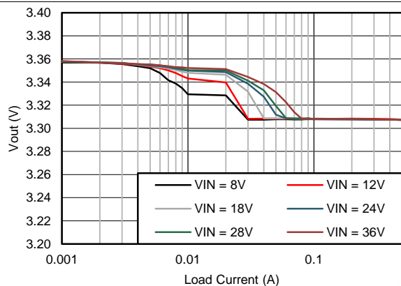
Figure 55. Output Voltage Regulation
