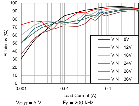
Figure 66. Efficiency
