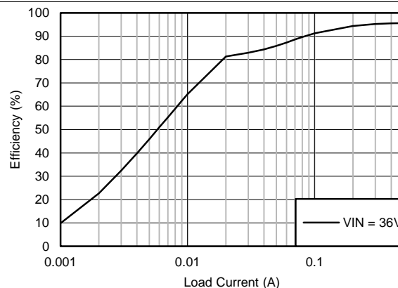
Figure 4. Efficiency
