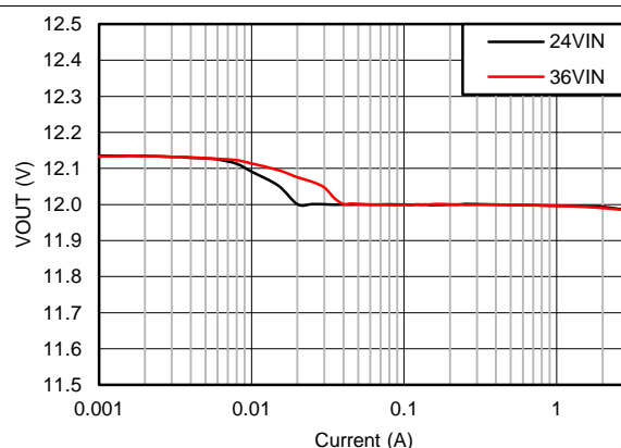
Figure 10. V_{OUT} Regulation
