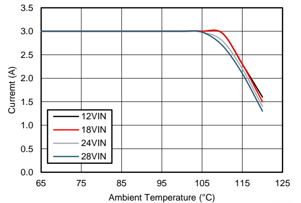
V_{OUT} = 5\text{ V} F_S = 200\text{ kHz} \theta_{JA} = 20^\circ\text{C/W}
