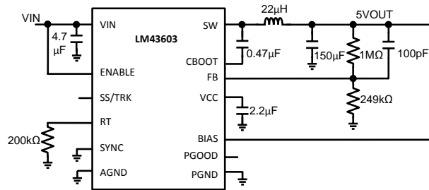
V_{OUT} = 5\text{ V} F_S = 200\text{ kHz}
