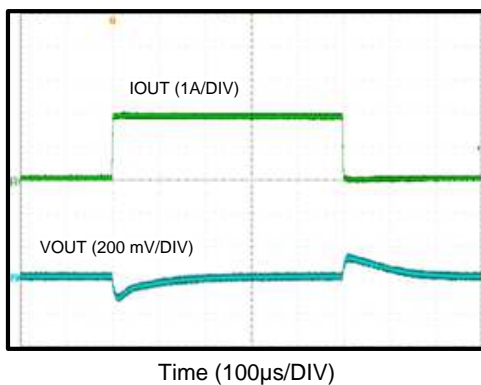
V_{OUT} = 5\text{ V} F_S = 200\text{ kHz}
