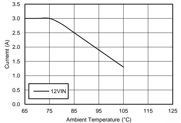
Figure 90. Derating Curve
