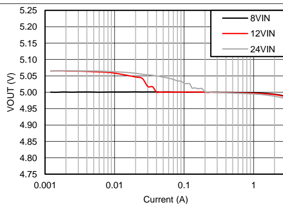
Figure 8. V_{OUT} Regulation
