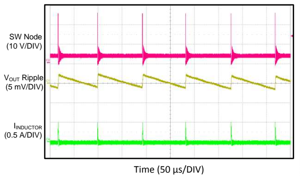
Figure 89. Switching Waveform in CCM Operation
