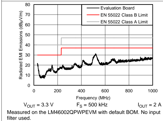
Figure 21. Radiated EMI Curve
