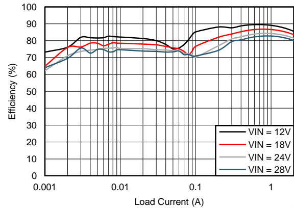
Figure 48. Efficiency
