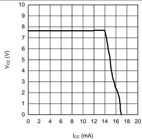
Figure 2. V_{CC} vs I_{CC} ( V_{IN} = 48\text{ V} )
