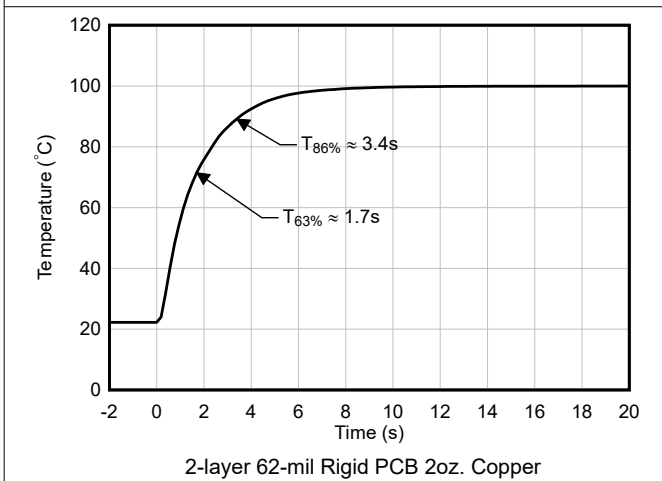
Figure 6-31. Thermal Response in Stirred Oil Bath (0.5 inches × 0.5 inches PCB board)
