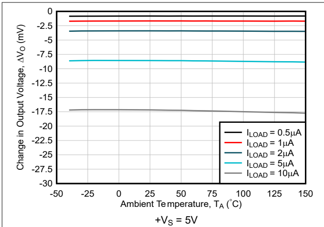
Figure 6-27. Load Regulation vs Ambient Temperature
