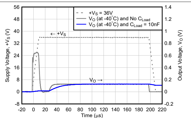
Figure 8-7. Start-up Response to +V_S = 36V Step Without C_{By-pass} When SR = 3.3V/\mu s (With No C_{Load} and C_{Load} = 10nF )
