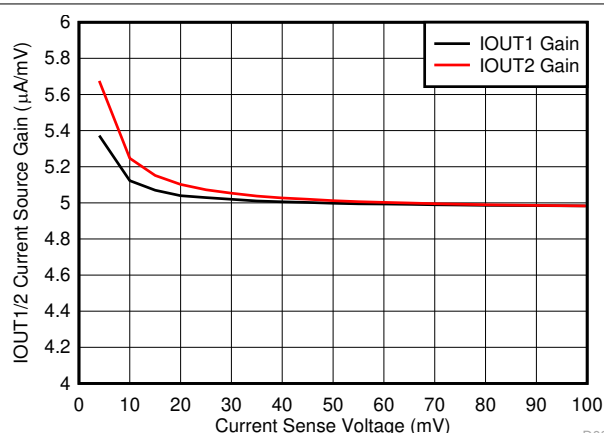
Figure 7-6. IOUT1/2 Current Monitor Accuracy vs V_{CS}
