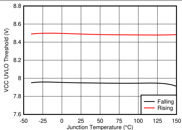
Figure 7-4. VCC UVLO Threshold vs Temperature
