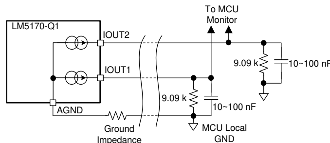
Figure 8-6. Channel Current Monitor
