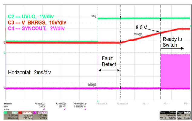
Figure 9-17. Start-Up Sequence Following UVLO Enable
