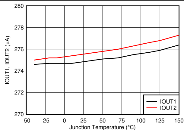
Figure 7-10. IOUT1/2 Current Monitor vs Temperature V_{CS} = 50 \text{ mV}
