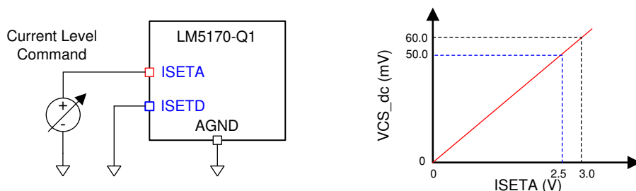
Figure 8-3. Pin Configurations for Current Setting Using an Analog Voltage Signal
