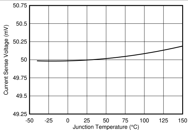
Figure 7-8. Regulated V_{CS} Voltage vs Temperature V_{ISETA} = 2.5 \text{ V}
