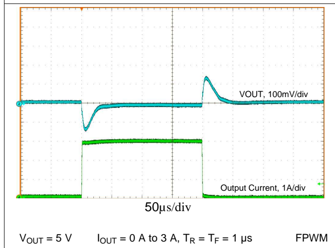
Figure 31. Load Transient
