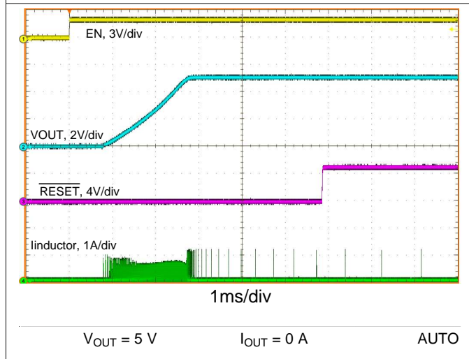
Figure 29. Start-up
