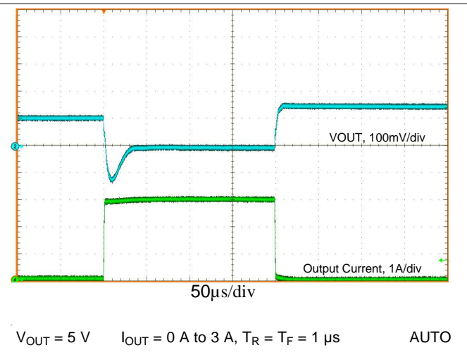
Figure 30. Load Transients
