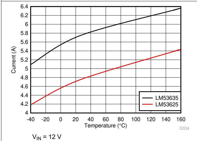
Figure 7-3. High Side/Peak Current Limit for LM53625/35-Q1
