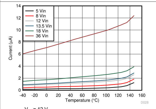
Figure 7-6. Shutdown Current
