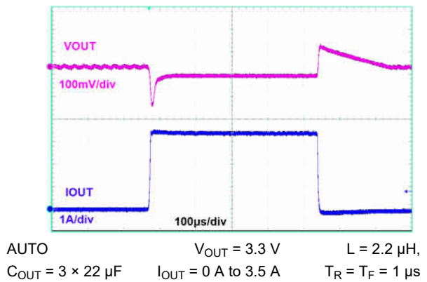
Figure 9-30. Load Transient
