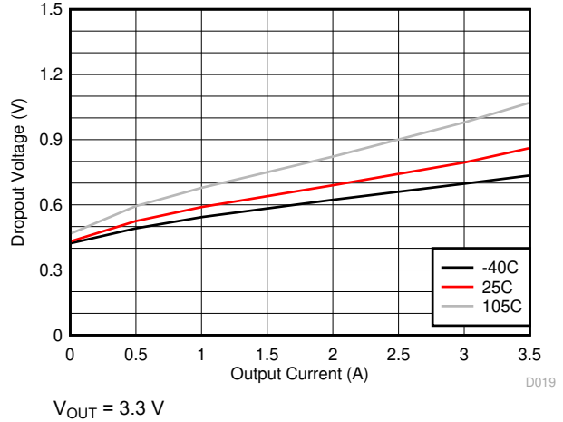
Figure 9-26. Dropout for \geq 1.85 MHz
