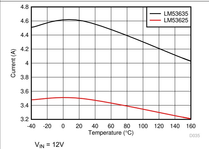
Figure 7-4. Low Side/Valley Current Limit for LM53625/35-Q1
