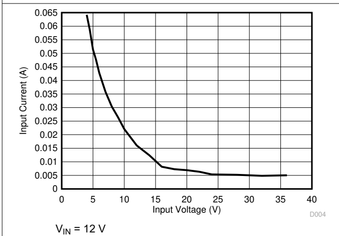
Figure 7-5. Short Circuit Average Input Current for LM53635-Q1
