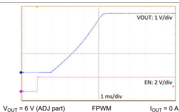
Figure 9-36. Start-up Waveform
