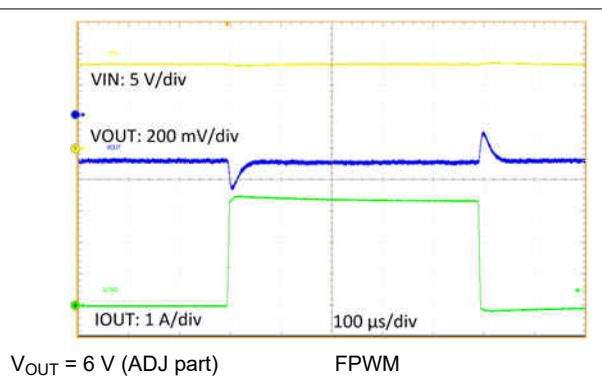
Figure 9-38. Load Transient
