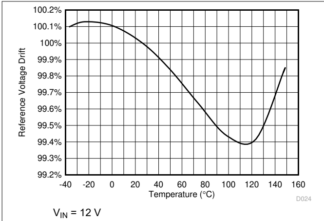
Figure 7-1. Reference Voltage Drift
