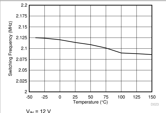
Figure 7-2. Switching Frequency vs Temperature
