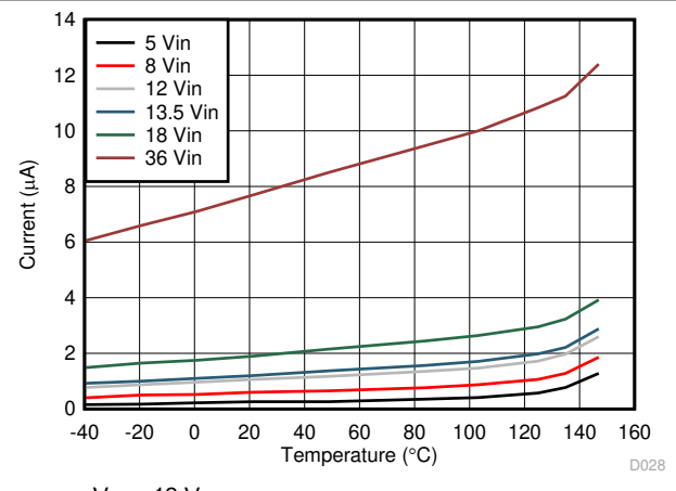
Figure 7-6. Shutdown Current
