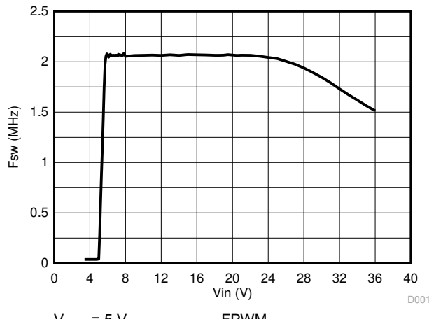
Figure 9-14. Switching Frequency vs Input Voltage
