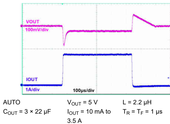
Figure 9-16. Load Transients
