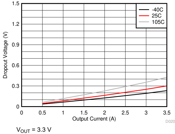
Figure 9-25. Dropout for -3% Regulation
