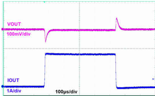
FPWM V_{OUT} = 3.3\text{ V} L = 2.2\ \mu\text{H} , C_{OUT} = 3 \times 22\ \mu\text{F} I_{OUT} = 0\ \text{A to } 3.5\ \text{A} T_R = T_F = 1\ \mu\text{s}
