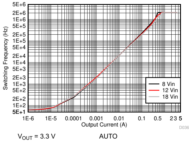
Figure 9-27. Switching Frequency vs Load Current
