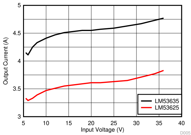
Figure 9-15. Output Current Level Limit Before Overcurrent Protection
