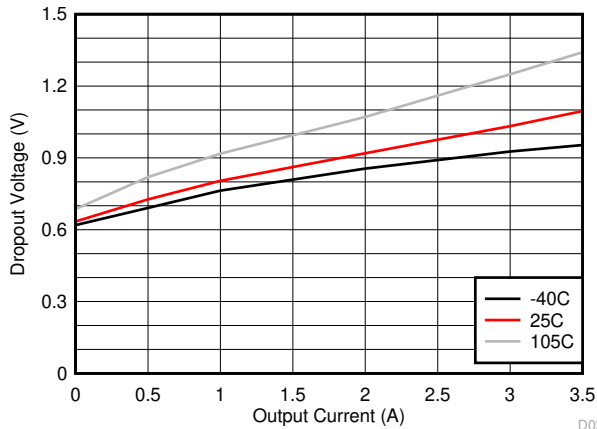
Figure 9-12. Dropout for \geq 1.85\text{ MHz}
