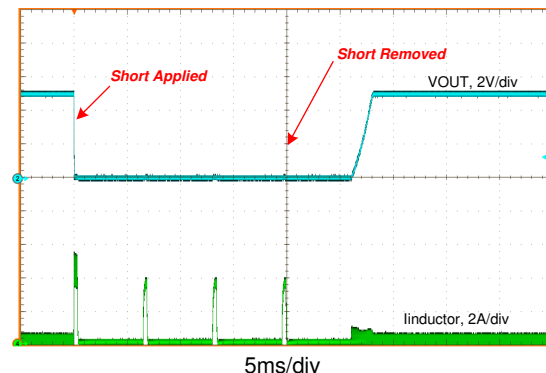
Figure 8-6. Short-Circuit Transient and Recovery
