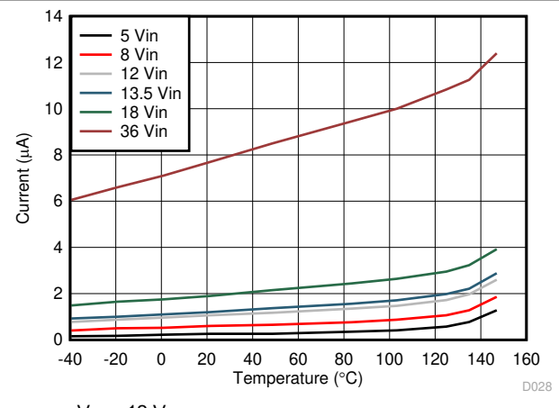
Figure 7-6. Shutdown Current
