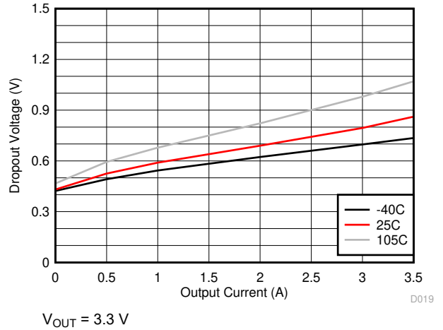
Figure 9-26. Dropout for \geq 1.85 MHz
