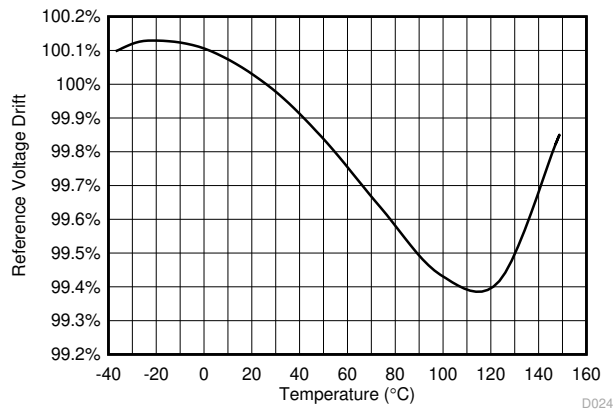
Figure 7-1. Reference Voltage Drift
