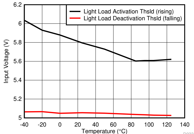
Figure 8-9. Input Voltage for Mode Change — Fixed 5-V Output, 2.2-µH Inductor
