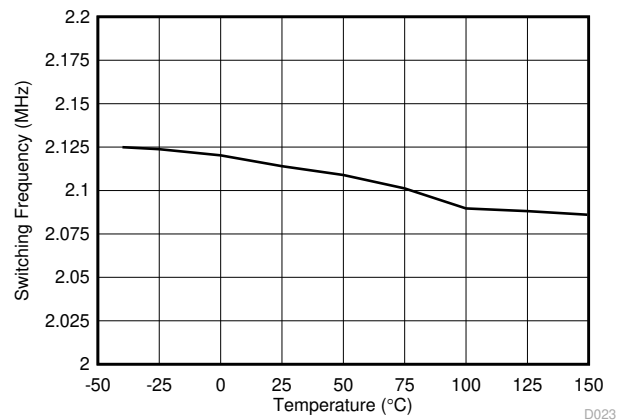
Figure 7-2. Switching Frequency vs Temperature
