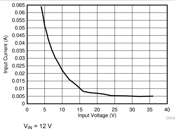
Figure 7-5. Short Circuit Average Input Current for LM53635-Q1
