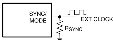
Figure 8-13. Frequency Synchronization
