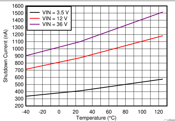
Figure 7-2. Shutdown Quiescent Current
