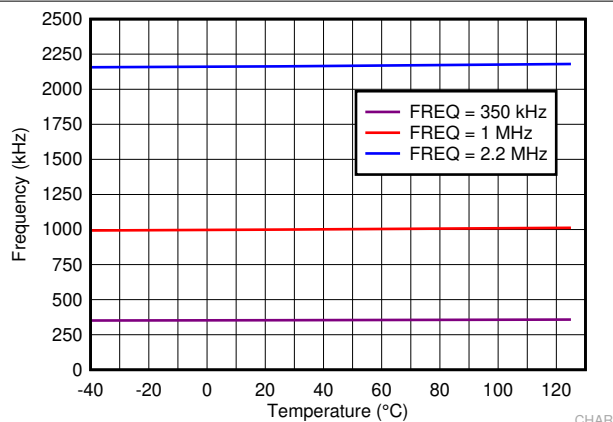
Figure 7-6. Switching Frequency Set by R_T Resistor
