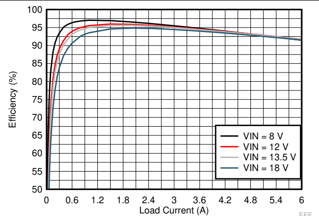
Figure 9-10. LM73605-Q1 Efficiency
