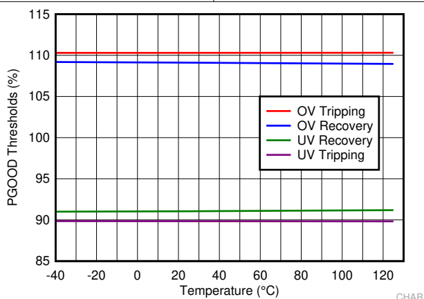
Figure 7-9. PGOOD Thresholds
