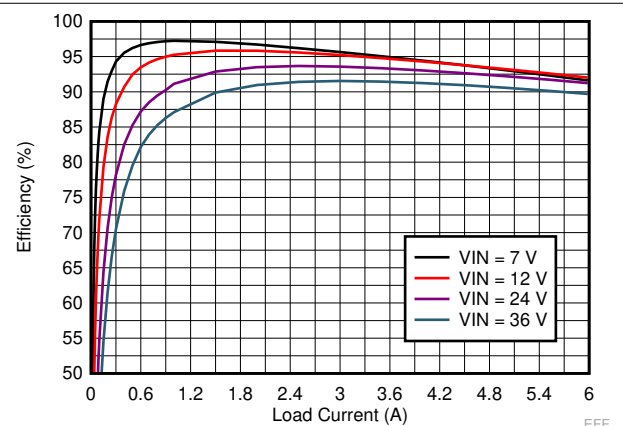
Figure 9-12. LM73606-Q1 Efficiency
