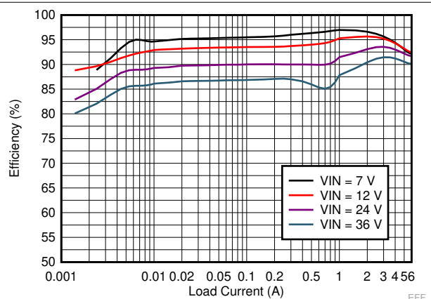
Figure 9-11. LM73606-Q1 Efficiency
