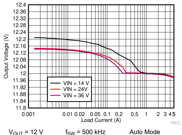
Figure 9-33. LM73605-Q1 Load and Line Regulation
