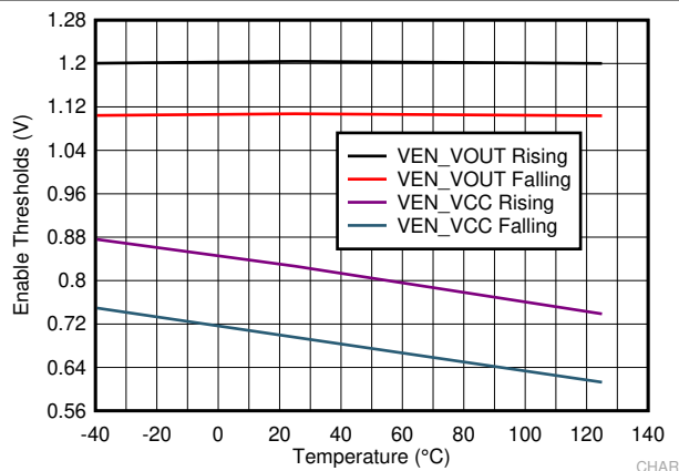
Figure 7-8. Enable Thresholds
