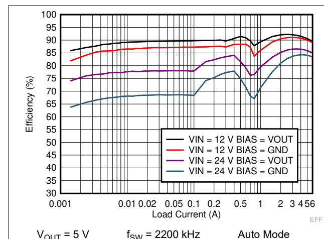
Figure 8-6. LM73606-Q1 Efficiency Comparison With Bias = V OUT to Bias = GND in Auto Mode
