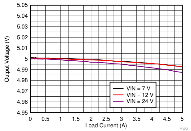
Figure 9-24. LM73606-Q1 Load and Line Regulation
