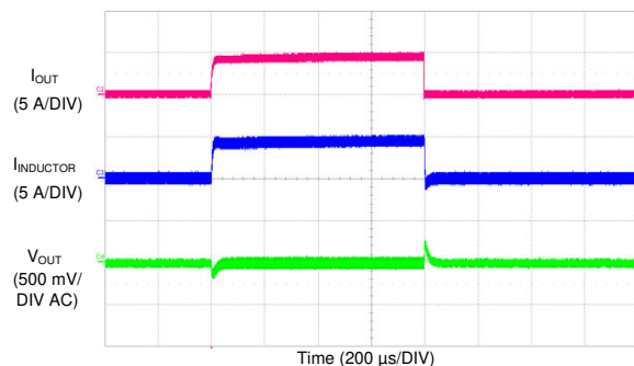
Figure 9-58. LM73606-Q1 Load Transients
