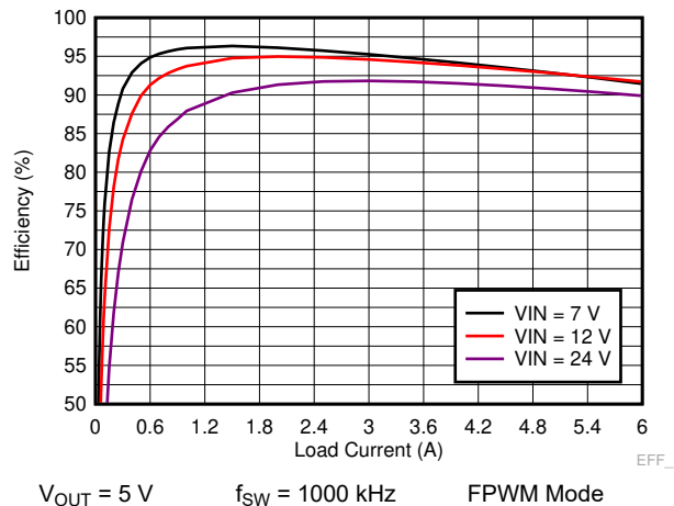
Figure 9-16. LM73606-Q1 Efficiency
