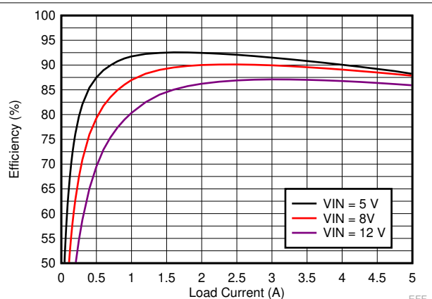
Figure 9-6. LM73605-Q1 Efficiency
