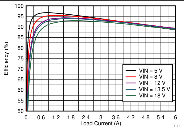
Figure 9-4. LM73606-Q1 Efficiency
