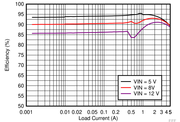
Figure 9-10. LM73605-Q1 Efficiency
