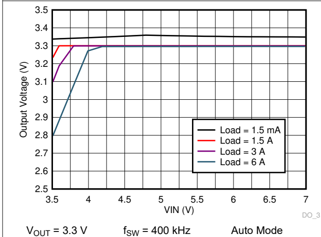
Figure 9-41. LM73606-Q1 Dropout Curve
