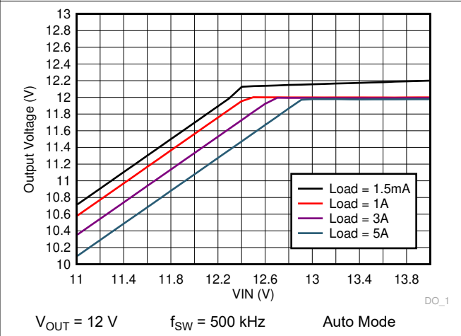
Figure 9-44. LM73605-Q1 Dropout Curve
