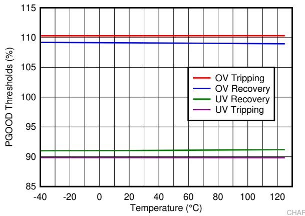
Figure 7-9. PGOOD Thresholds
