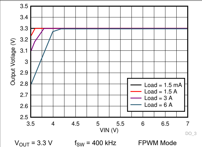
Figure 9-42. LM73606-Q1 Dropout Curve
