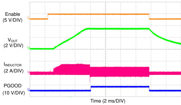
Figure 9-51. LM73606-Q1 Overcurrent Behavior
