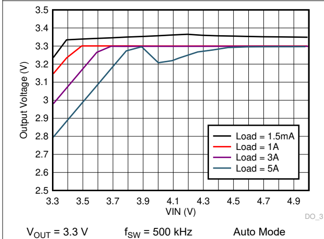
Figure 9-43. LM73605-Q1 Dropout Curve
