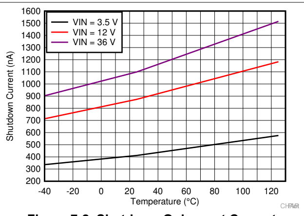
Figure 7-2. Shutdown Quiescent Current
