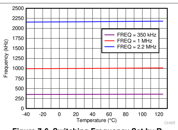
Figure 7-6. Switching Frequency Set by R_T Resistor
