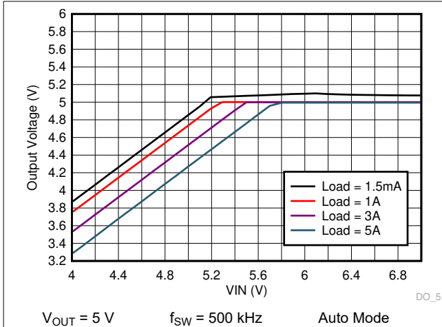
Figure 9-39. LM73605-Q1 Dropout Curve
