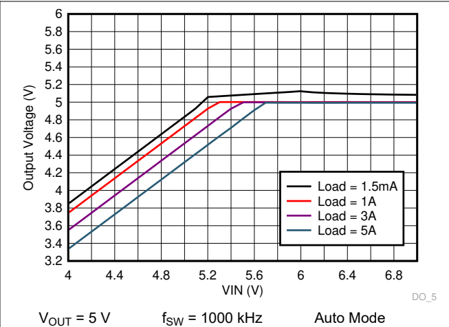
Figure 9-40. LM73605-Q1 Dropout Curve
