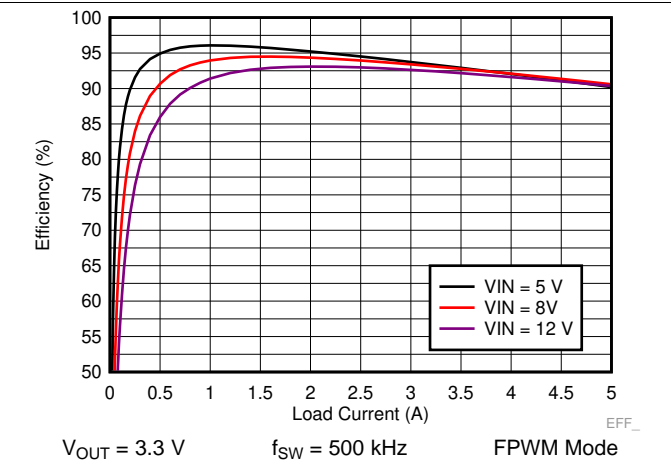
Figure 28. LM73605 Efficiency
