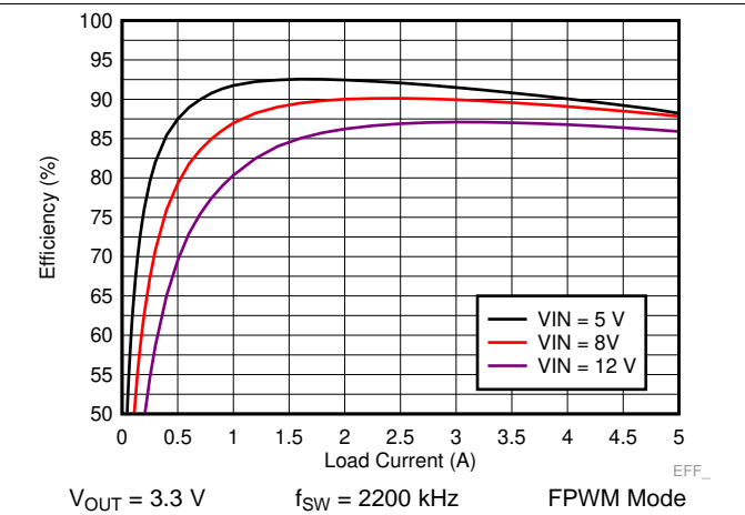
Figure 30. LM73605 Efficiency
