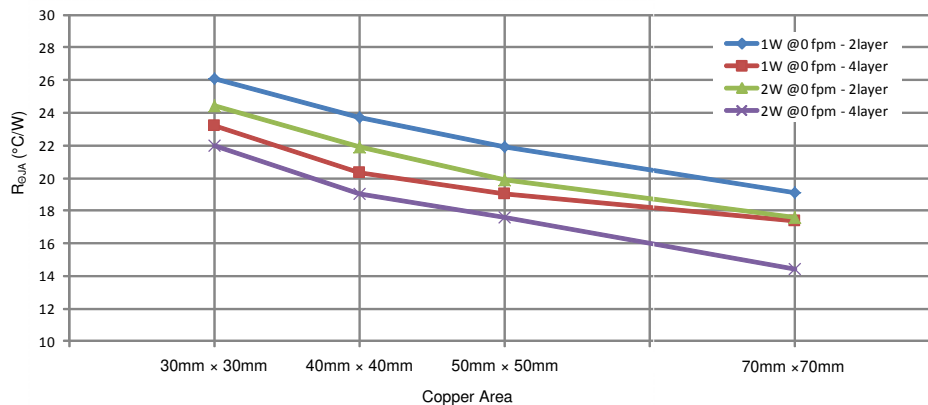
Figure 76. Measured R_{\theta JA} versus PCB Copper Area on 2-Layer Boards and 4-Layer Boards
