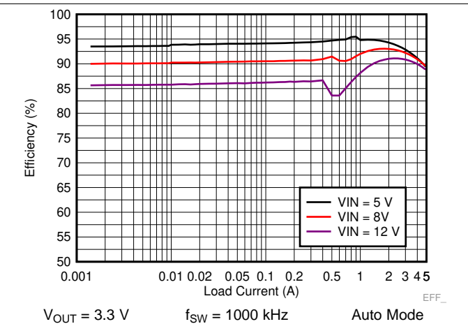
Figure 32. LM73605 Efficiency
