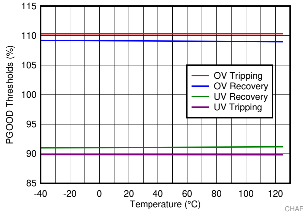
Figure 9. PGOOD Thresholds
