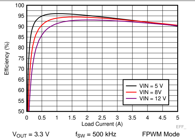
Figure 28. LM73605 Efficiency
