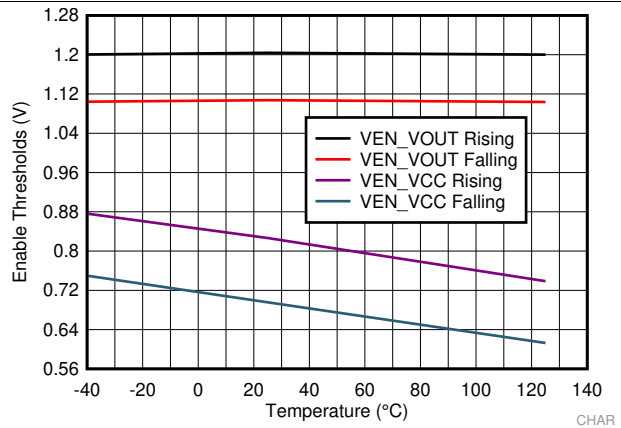
Figure 8. Enable Thresholds
