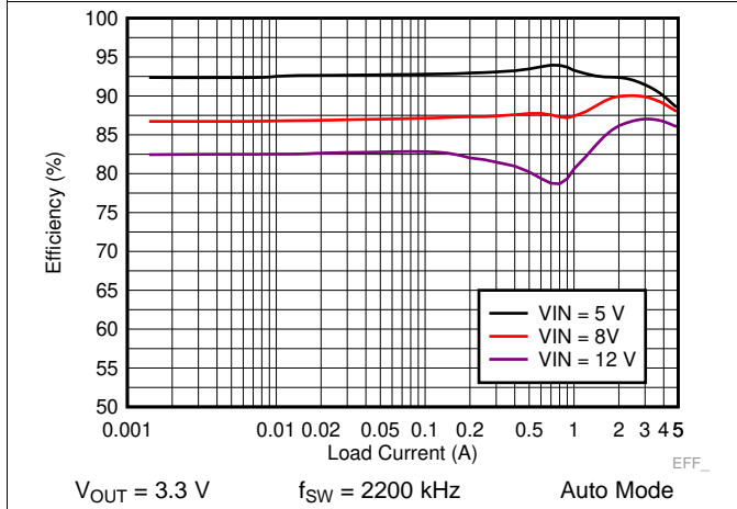
Figure 29. LM73605 Efficiency
