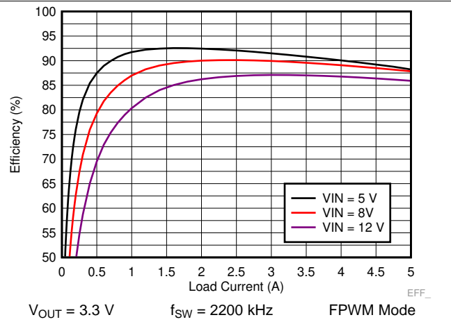
Figure 30. LM73605 Efficiency
