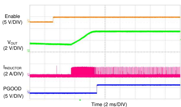
Figure 66. LM73606 Soft Start With 200-mA Load in Auto Mode
