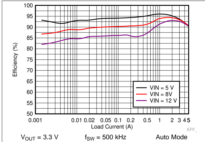
Figure 27. LM73605 Efficiency
