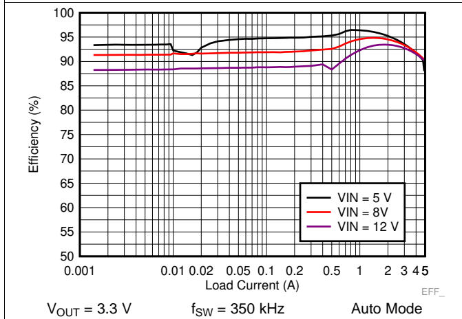
Figure 31. LM73605 Efficiency
