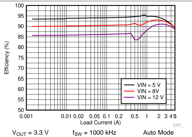
Figure 32. LM73605 Efficiency
