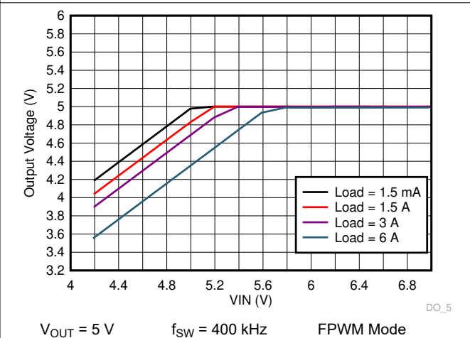
Figure 9-36. LM73606-Q1 Dropout Curve
