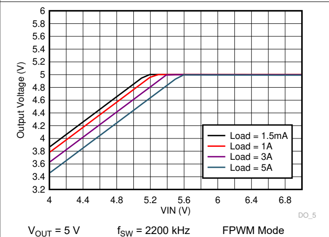
Figure 9-38. LM73605-Q1 Dropout Curve
