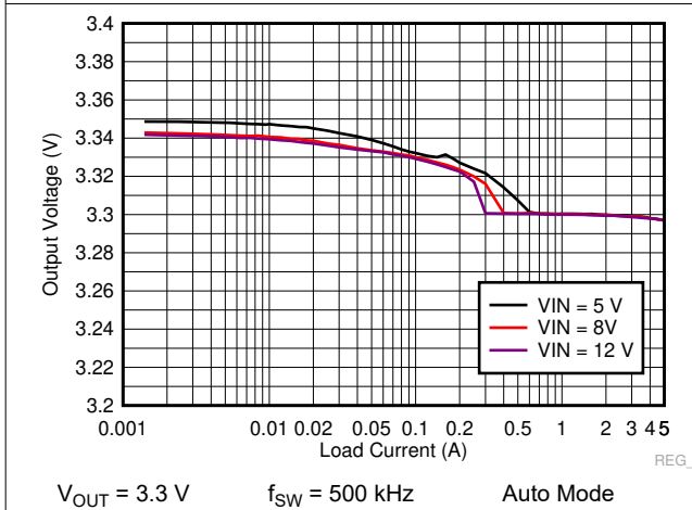
Figure 9-31. LM73605-Q1 Load and Line Regulation
