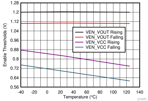
Figure 7-8. Enable Thresholds
