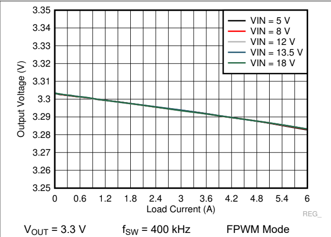
Figure 9-28. LM73606-Q1 Load and Line Regulation
