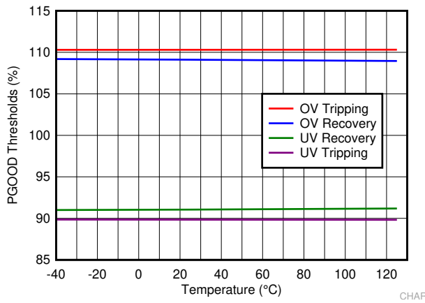
Figure 7-9. PGOOD Thresholds
