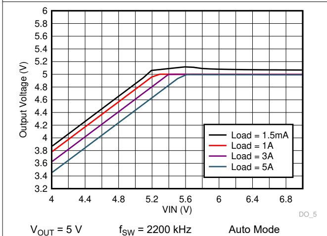
Figure 9-37. LM73605-Q1 Dropout Curve
