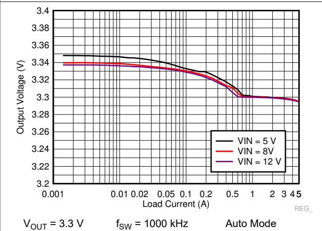
Figure 9-32. LM73605-Q1 Load and Line Regulation
