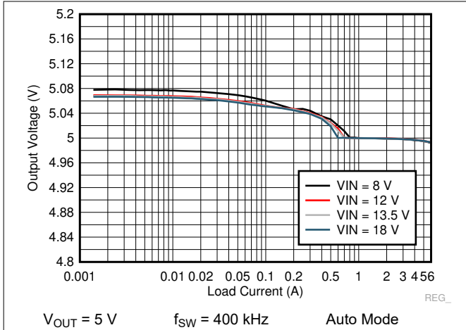
Figure 9-21. LM73606-Q1 Load and Line Regulation
