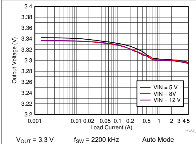
Figure 9-29. LM73605-Q1 Load and Line Regulation
