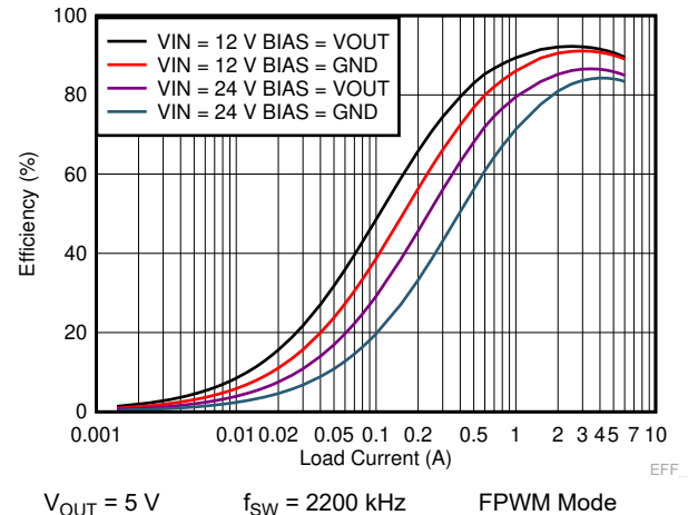
Figure 8-7. LM73606-Q1 Efficiency Comparison With Bias = V_{OUT} to Bias = GND in FPWM Mode
