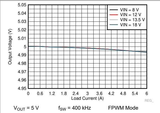
Figure 9-22. LM73606-Q1 Load and Line Regulation
