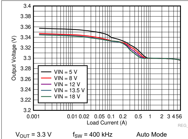
Figure 9-27. LM73606-Q1 Load and Line Regulation
