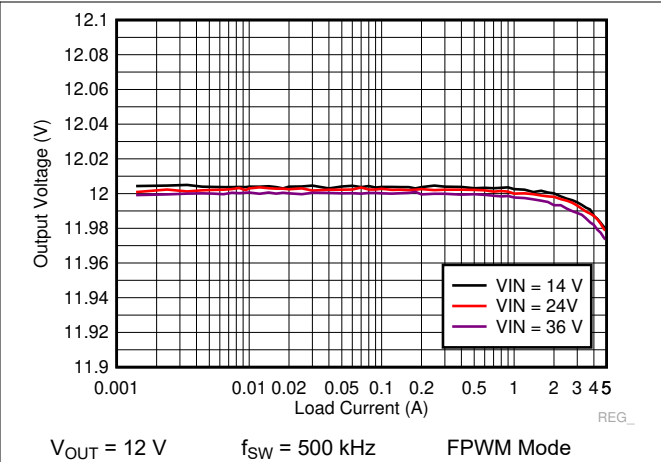
Figure 9-34. LM73605-Q1 Load and Line Regulation
