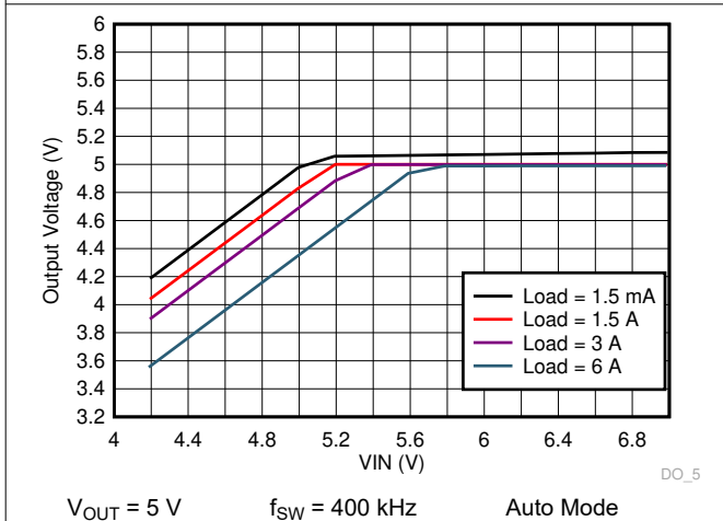
Figure 9-35. LM73606-Q1 Dropout Curve
