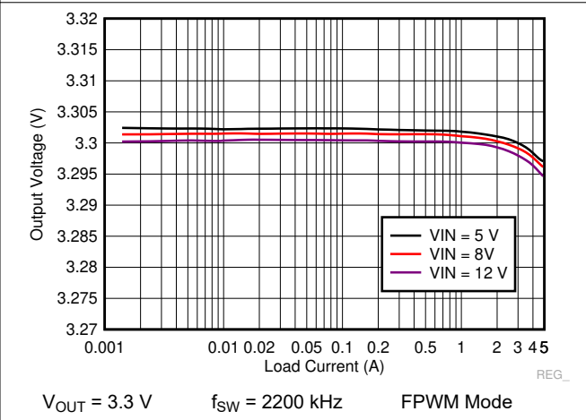
Figure 9-30. LM73605-Q1 Load and Line Regulation
