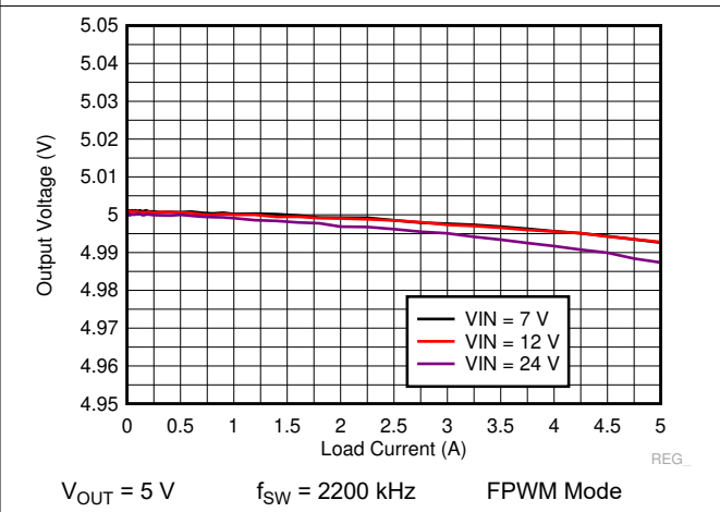
Figure 9-26. LM73605-Q1 Load and Line Regulation
