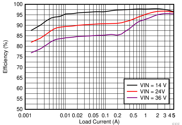
Figure 9-17. LM73606-Q1 Efficiency
