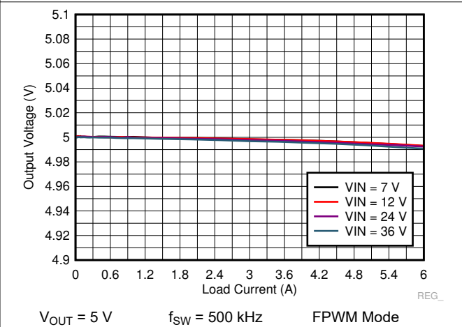
Figure 9-24. LM73606-Q1 Load and Line Regulation
