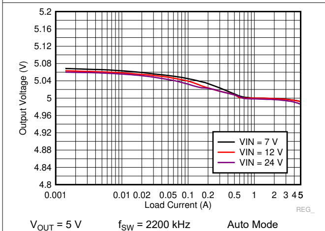
Figure 9-25. LM73605-Q1 Load and Line Regulation
