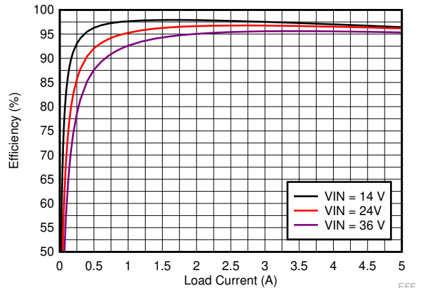
Figure 9-18. LM73606-Q1 Efficiency
