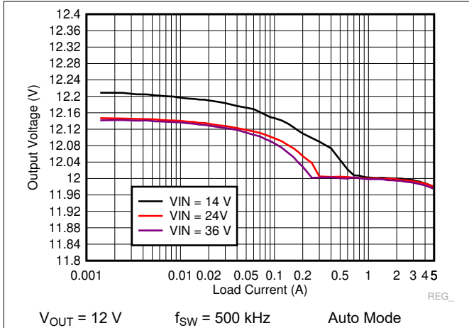
Figure 9-33. LM73605-Q1 Load and Line Regulation
