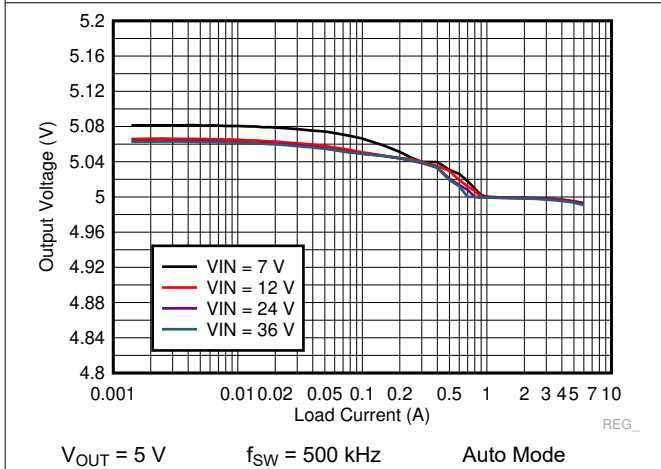
Figure 9-23. LM73606-Q1 Load and Line Regulation
