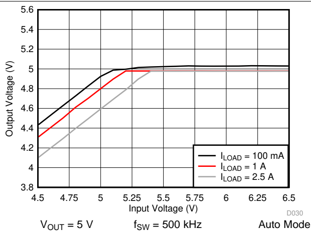
Figure 55. LM76002 Dropout Curve
