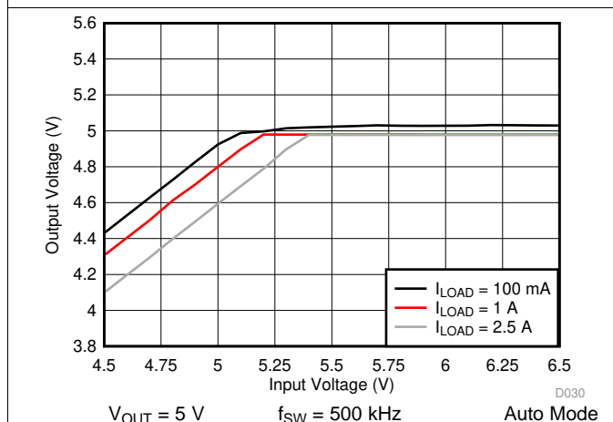
Figure 55. LM76002 Dropout Curve
