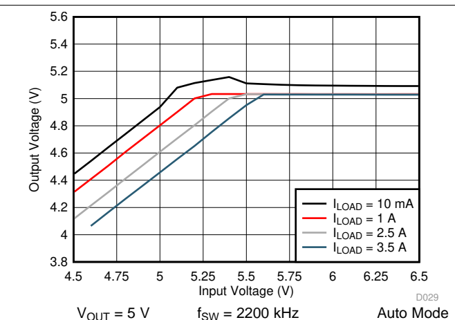
Figure 54. LM76003 Dropout Curve
