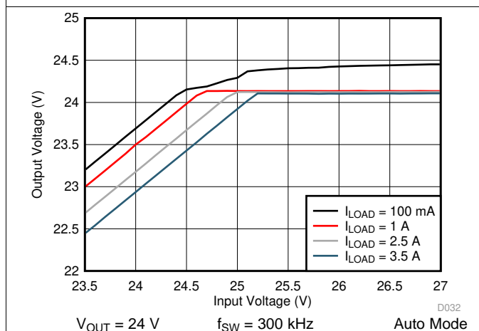
Figure 57. LM76003 Dropout Curve
