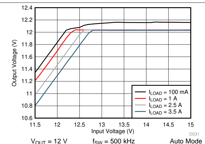
Figure 56. LM76003 Dropout Curve
