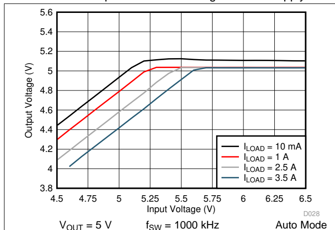
Figure 53. LM76003 Dropout Curve
