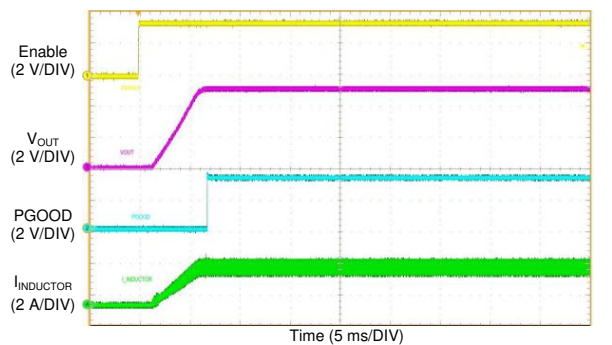
Figure 67. Start-up Waveform
