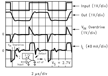
Figure 53. Buffer Amplifier Scope Photo
