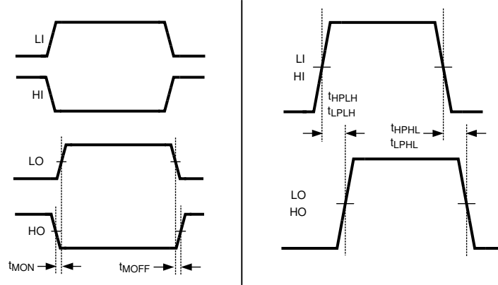
Figure 6-1. Timing Diagram
