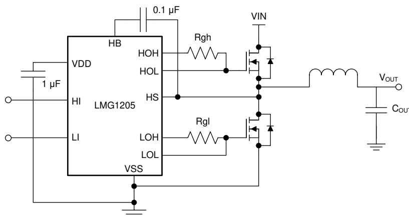
Figure 8-1. Application Circuit
