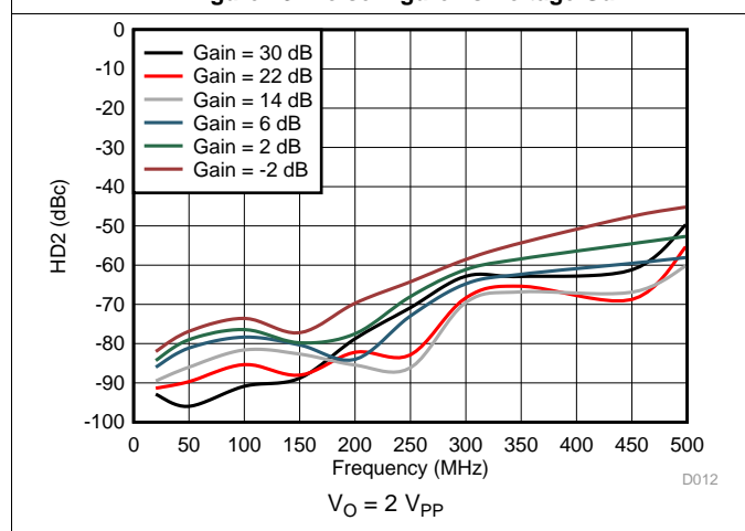
Figure 15. HD2 vs Frequency and Gain Settings
