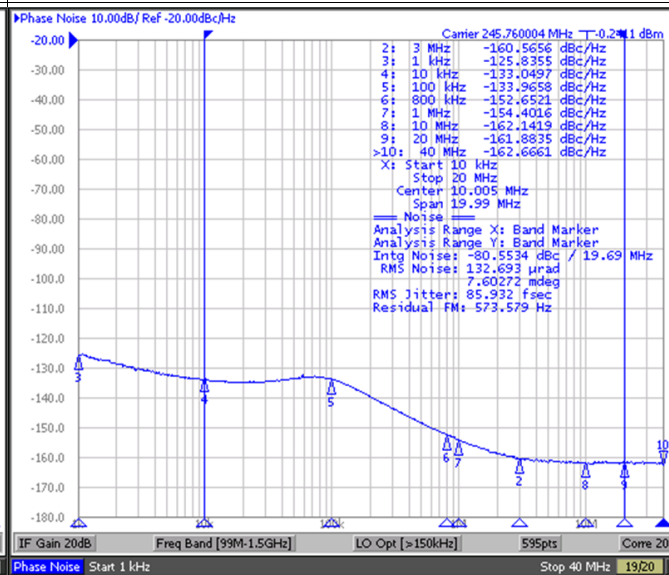
Figure 3. LMK04821 DCLKout2 Phase Noise
