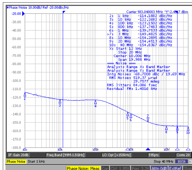
Figure 34. DCLKout4, 983.04-MHz LVPECL16 With 240-Ω Emitter Resistors CLKout4_5_IDL = 1, CLKout4_5_ODL = 0
