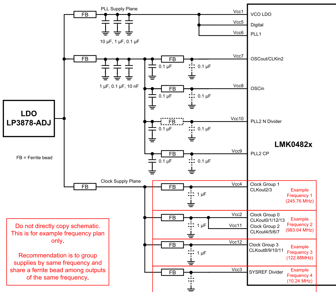
Figure 41. Example Application - Power System Schematic
