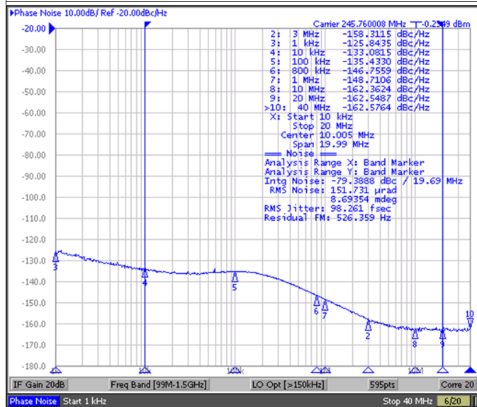
Figure 2. LMK04821 DCLKout2 Phase Noise
