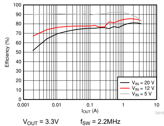
Figure 5-4. Efficiency vs. Load Current
