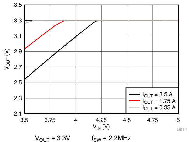
Figure 5-10. Dropout Curve
