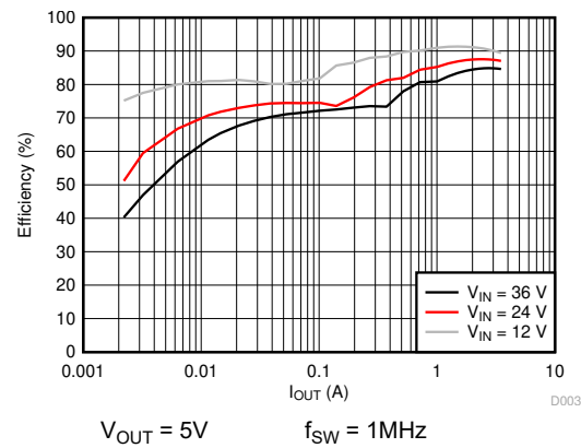
Figure 5-2. Efficiency vs. Load Current
