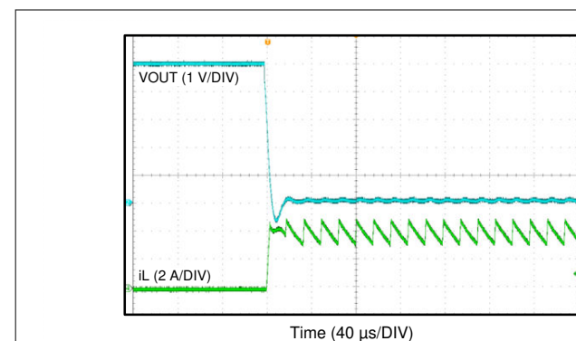
Figure 7-8. Output Short
