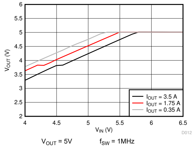
Figure 5-8. Dropout Curve
