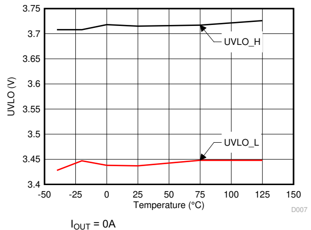
Figure 5-12. UVLO Threshold
