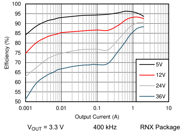
Figure 9-14. Efficiency
