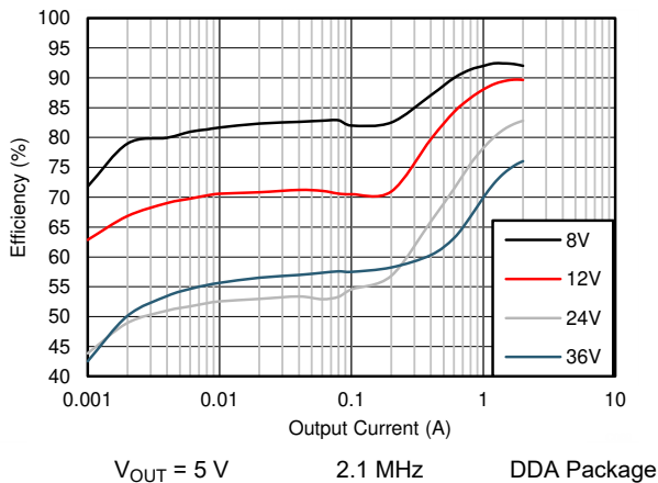
Figure 9-11. Efficiency
