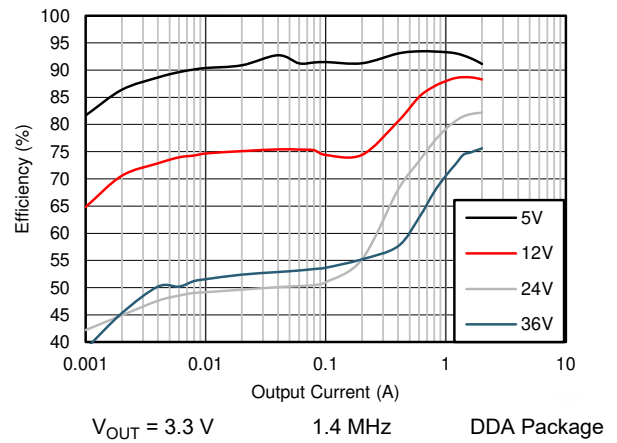
Figure 9-10. Efficiency
