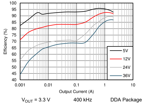
Figure 9-8. Efficiency
