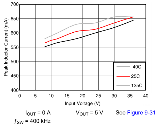
Figure 7-6. I_{PEAK-MIN}
