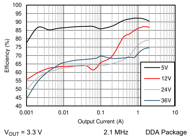
Figure 9-12. Efficiency
