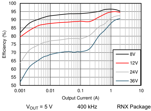
Figure 9-13. Efficiency
