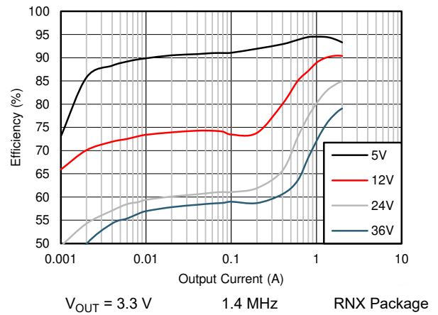
Figure 9-16. Efficiency
