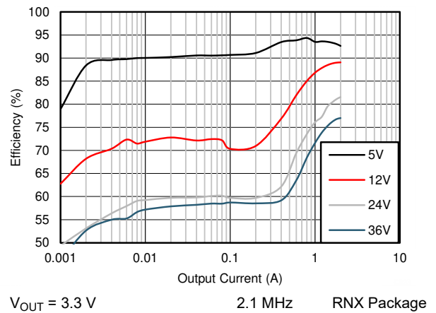
Figure 9-18. Efficiency
