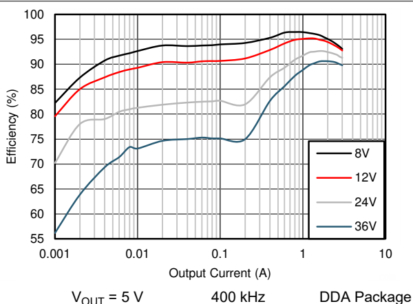
Figure 9-7. Efficiency
