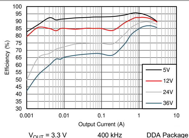
Figure 9-8. Efficiency
