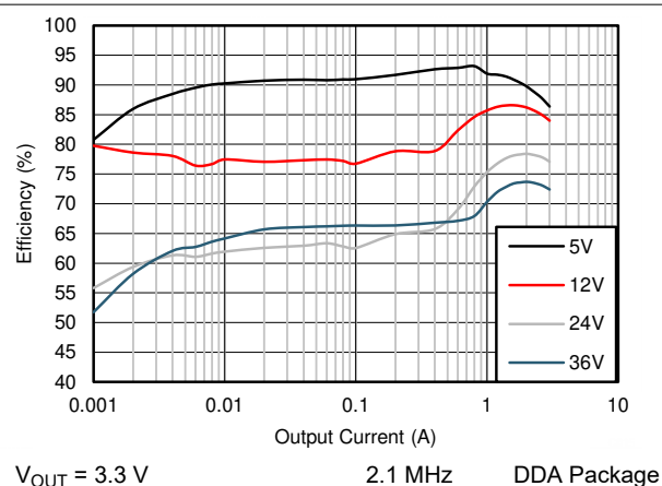
Figure 9-12. Efficiency
