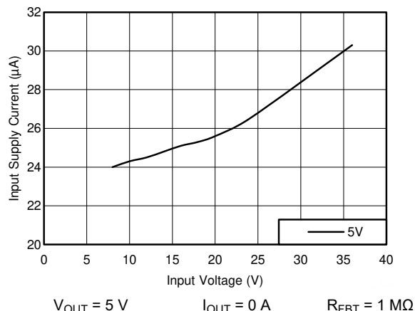
Figure 9-20. Input Supply Current
