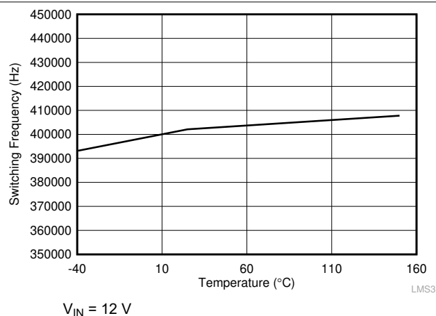
Figure 7-2. Switching Frequency vs Temperature
