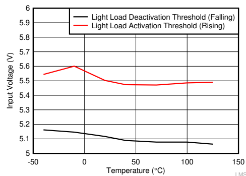
Figure 8-9. Input Voltage for Mode Change — 5-V Output, 10- \mu H Inductor
