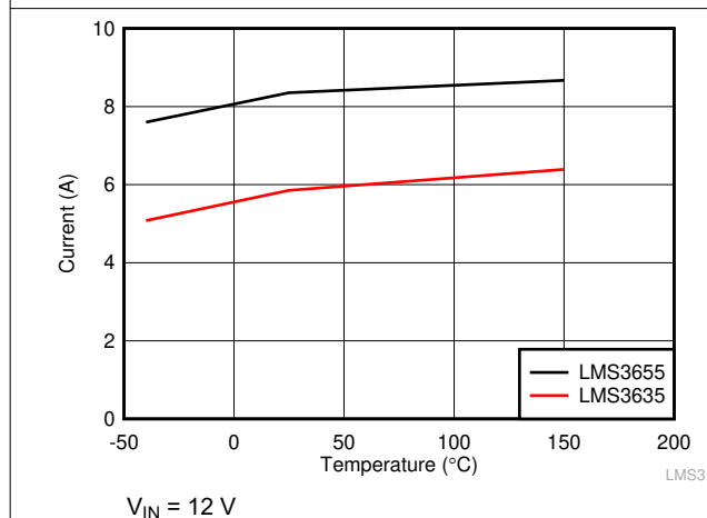
Figure 7-3. High-Side/Peak Current Limit for LMS36x5-Q1
