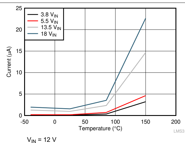
Figure 7-6. Shutdown Current
