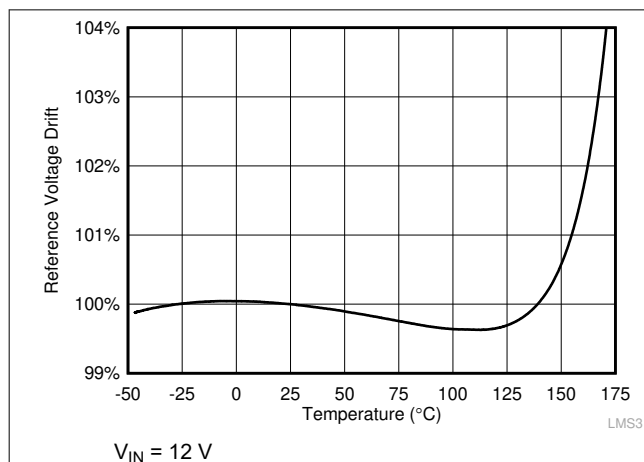
Figure 7-1. Reference Voltage Drift
