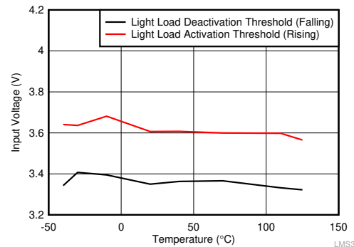
Figure 8-8. Input Voltage for Mode Change — 3.3-V Output, 10- \mu H Inductor
