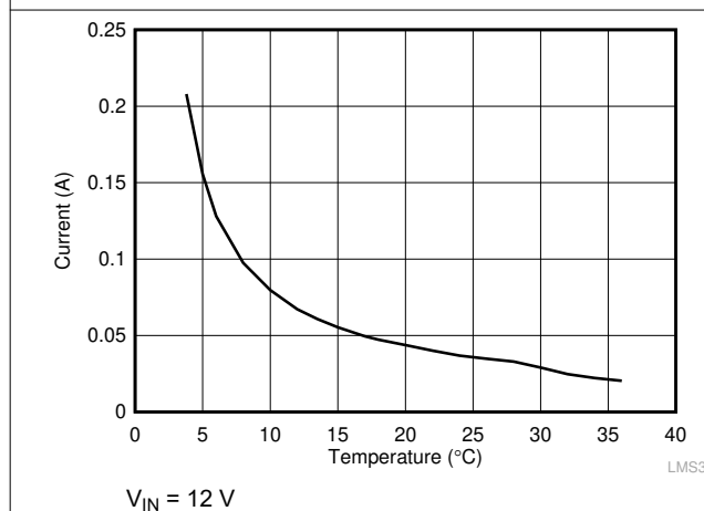
Figure 7-5. Short Circuit Average Input Current for LMS3635-Q1
