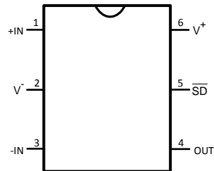
Pin Functions for SOT-23
